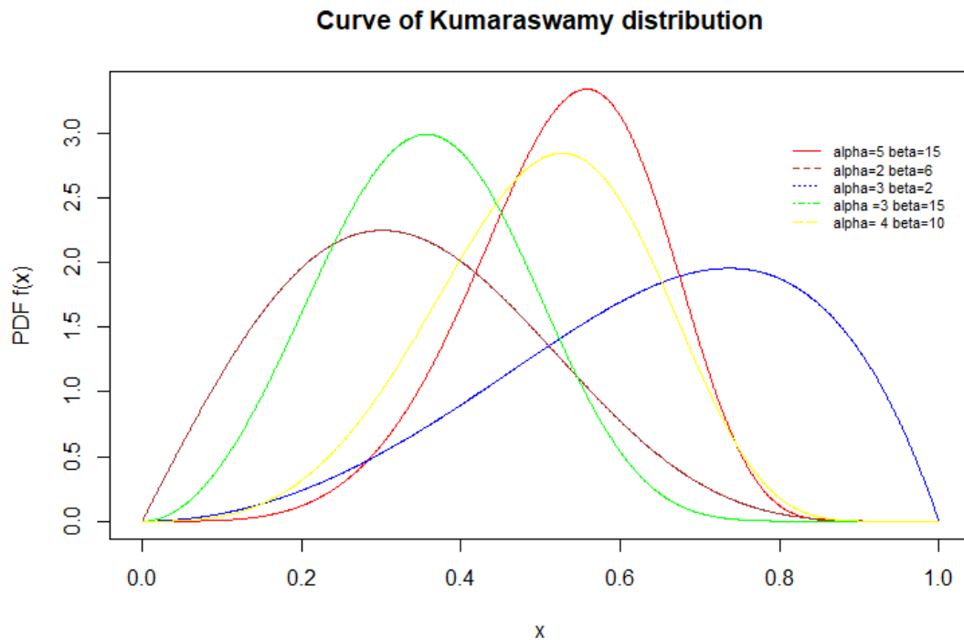
Figure 1: Probability Distribution Function curve of the Kumaraswamy under different parameters combinations.
