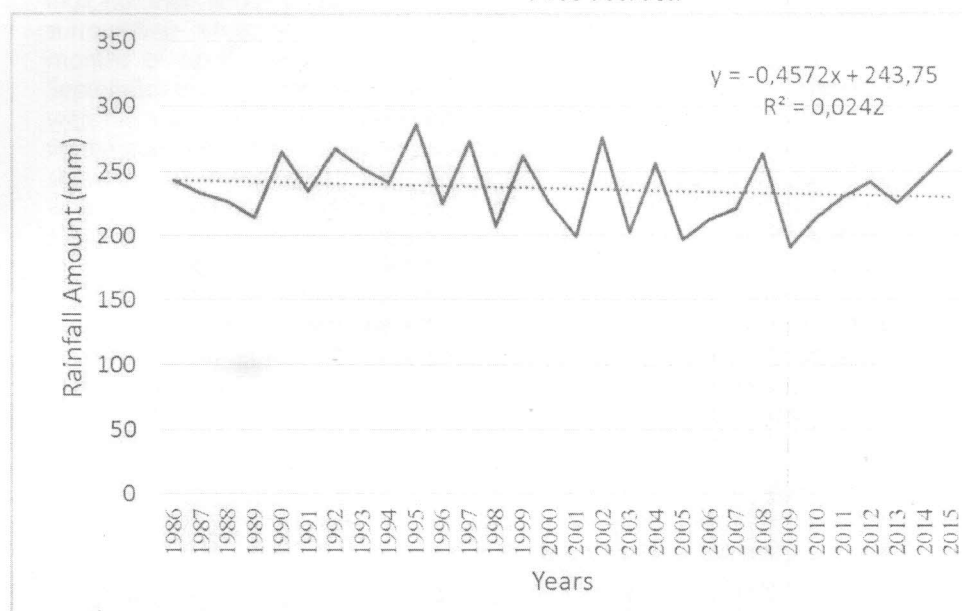
Fig. 4. Mean Rainfall Trend in Warri (1986-2015) (Authors' Computation 2017)
