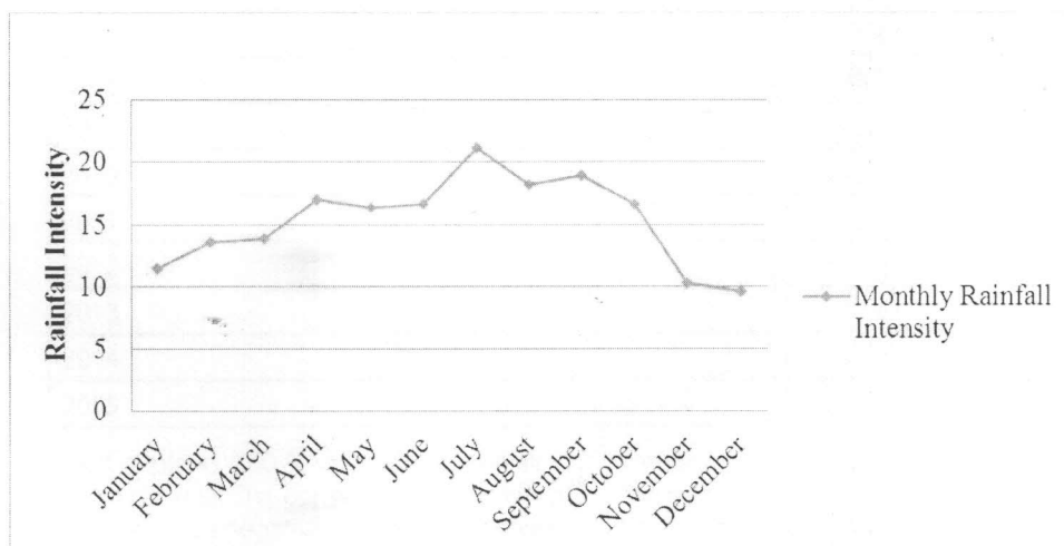
Fig. 3. Mean Monthly Rainfall Intensity in Warri Metropolis from 1986-2015 (Authors' Computation 2017)
