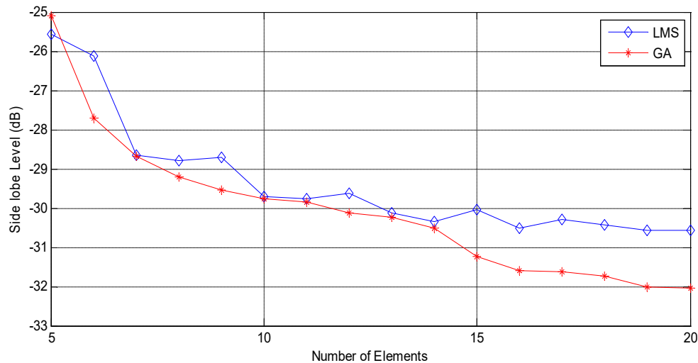
Figure 7: Comparison of LMS and GA Side Lobe level Results Obtained for Equally Spaced Antenna Elements
