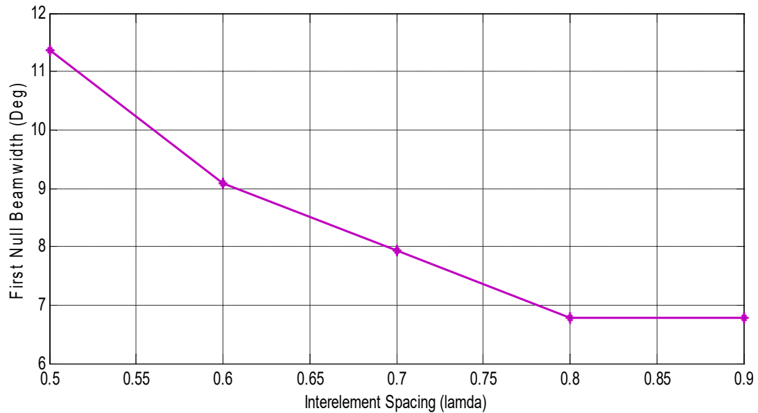
Figure 9: Result showing the effect of increase in Inter Element Spacing on Beamwidth
