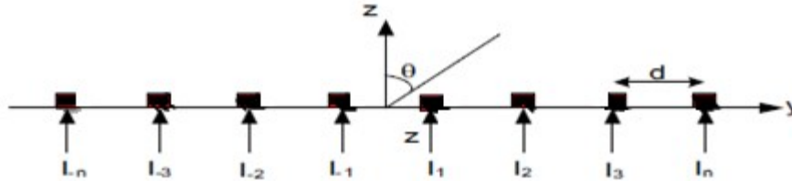
Figure 1: Equally Spaced Linear Array Arrangement [12]
