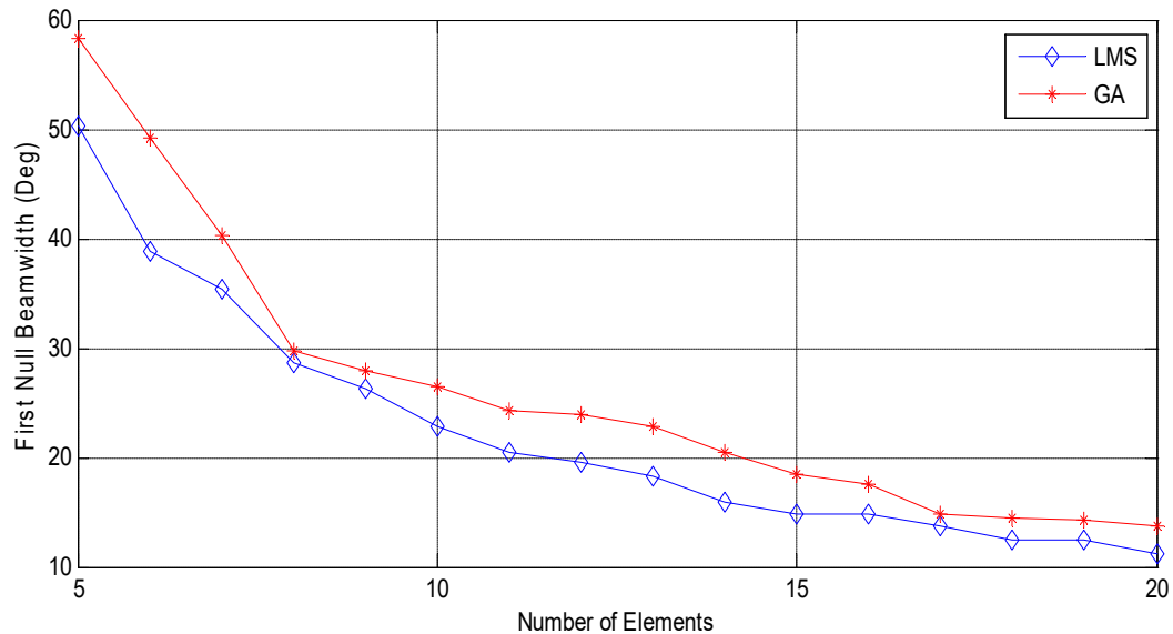
Figure 8: Comparison of LMS and GA Beamwidth Results Obtained for Equally Spaced Antenna Elements
