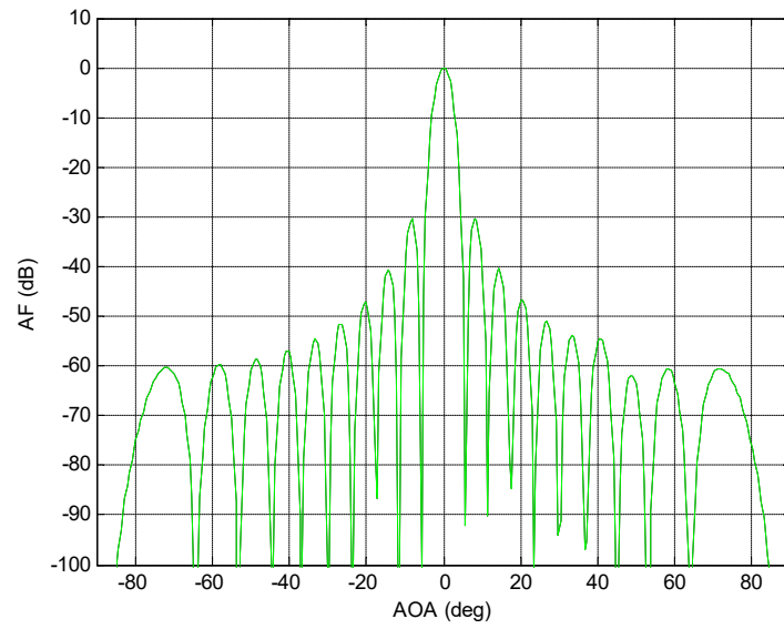
Figure 4: Radiation pattern for 20 Elements using LMS Algorithm
