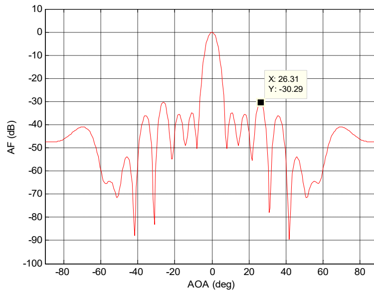
Figure 5: Radiation pattern for 18 Elements using GA
