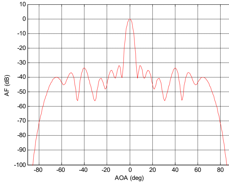
Figure 6: Radiation pattern for 20 Elements using GA
