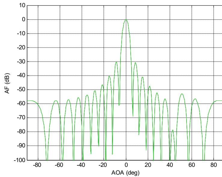
Figure 3: Radiation pattern for 19 Elements using LMS Algorithm
