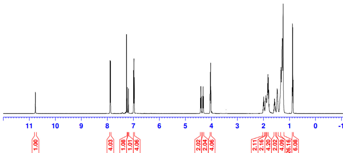
Fig. 3. ^1\text{H} NMR spectrum of compound 8 (in \text{CDCl}_3 ).
