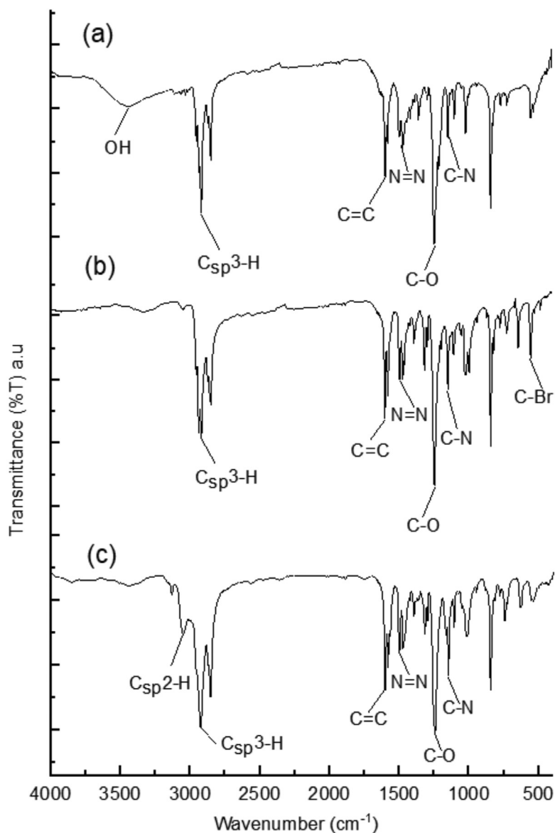
Fig. 1. FTIR spectra of compounds (a) 3 , (b) 6 and (c) 8 .
