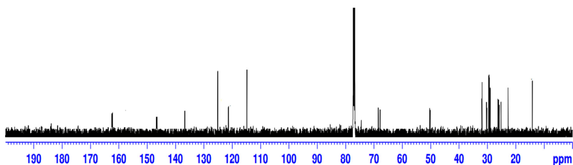
Fig. 4. ^{13}\text{C} NMR spectrum of compound 8 (in \text{CDCl}_3 ).
