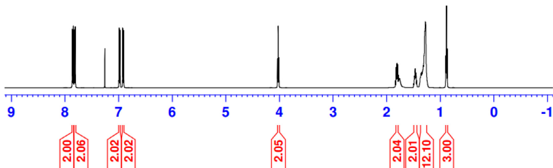
Fig. 2. ^1\text{H} NMR spectrum of compound 3 (in \text{CDCl}_3 ).
