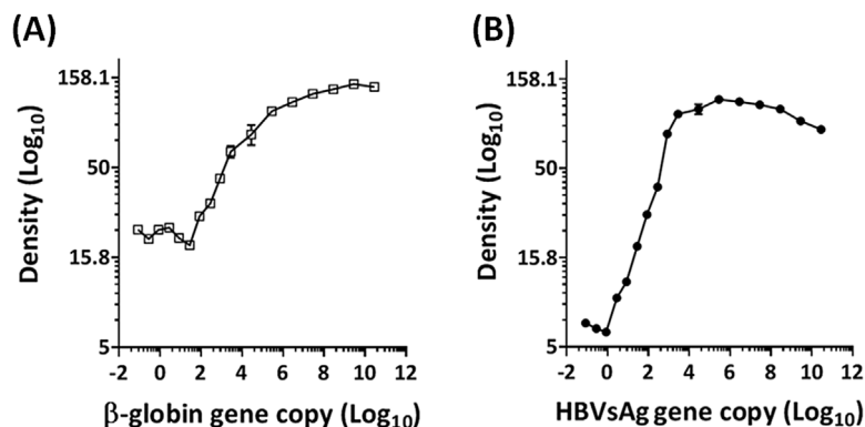
FIGURE 2 Input copy numbers assay showing densitometric plots of \beta -globin and HBs genes. In order to determine the linear ranges of conventional PCR for (A) \beta -globin and (B) HBs gene, the respective genes were amplified by PCR from a serial dilution of cloned targets with logarithmic increments in genome number. PCR amplicon was run through 2% agarose gel and DNA bands quantified by densitometry ( n = 2 \pm \text{S.E.M} )
