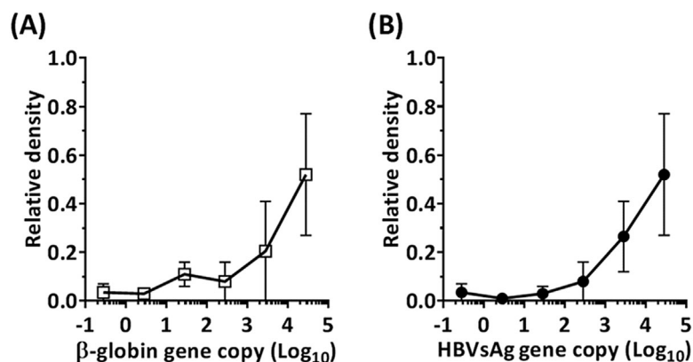
FIGURE 3 Mixed primers competition assays. To determine the effects of multiplex primers on PCR efficiency either (A) human \beta -globin or (B) HBsAg was amplified in a multiplex reaction containing equal concentrations of \beta -globin and HBsAg -specific primers. PCR products were analysed by agarose gel electrophoresis and DNA bands quantified by densitometry ( n = 2 \pm \text{S.E.M} )
