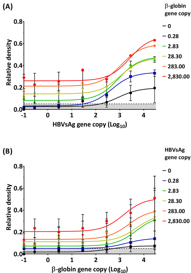
FIGURE 4 Multiplex PCR of \beta -globin and HBsAg with increasing genome copies. (A) Multiplex PCR of HBVsAg with increasing input copy number of \beta -globin. (B) Multiplex PCR of \beta -globin with increasing input copy number of HBVsAg. Both PCR amplicons were analysed by gel electrophoresis and DNA bands quantified by densitometry. A positive PCR was determined as having a relative density of above 0.05, based upon the data from the mixed primer competition assays. For clarity the area of the graph below 0.05 is shaded grey. ( n = 2 \pm \text{S.E.M} )
