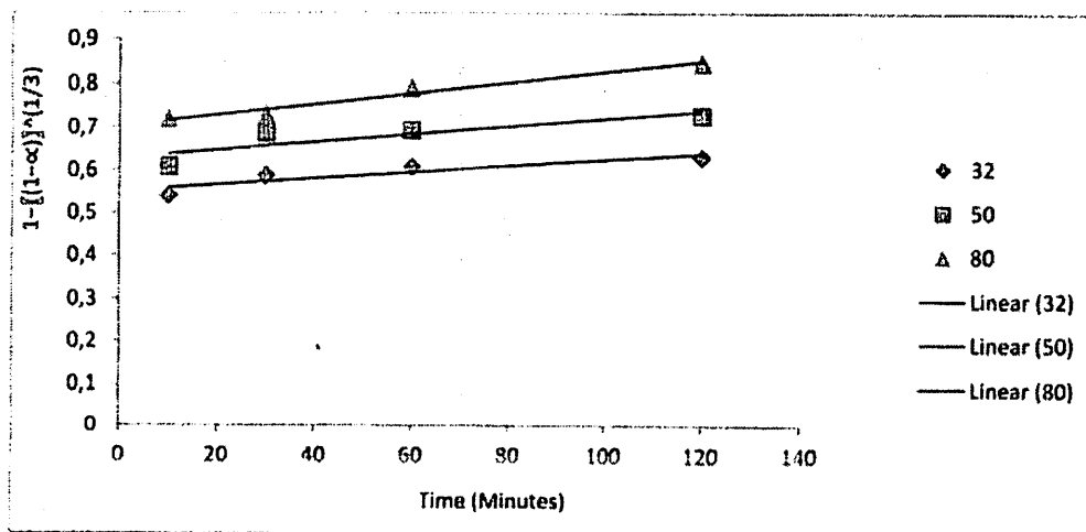
Fig. 10. Plot of 1 - (1 - \alpha)^{1/3} vs. leaching time at different temperature.
