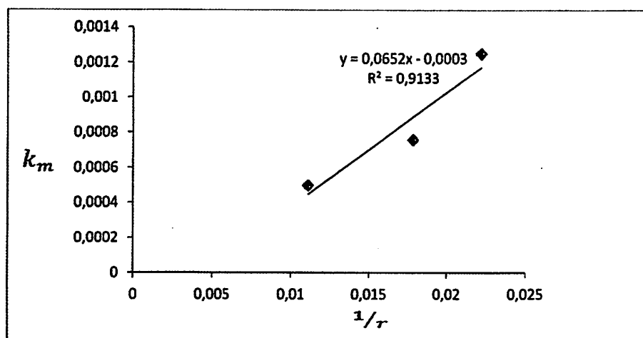
Fig. 12. Plot of K_m vs. (1/r) .
