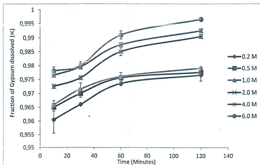
Fig. 4. Plot of fraction of gypsum dissolved versus leaching time at different concentrations of HCl. (Experimental conditions: solid-liquid ratio: 10 g/l; stirring rate: 400 rpm; particle size: - 90 + 63 \mu\text{m} ; temperature: 80°C).
