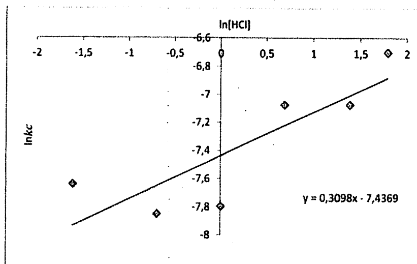
Fig. 9. Plot of \ln K_c against \ln[\text{HCl}] .
