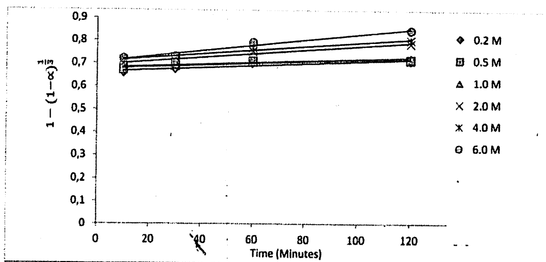
Fig. 8. Plot of 1 - (1 - \alpha)^{1/3} vs. leaching time at different HCl concentration.
