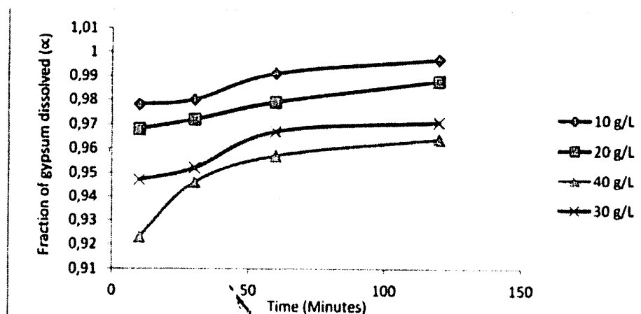
Fig. 7. Plot of fraction of gypsum dissolved versus leaching time at different solid-liquid ratio. (Experimental conditions: particle size: -90 + 63 \mu\text{m} ; [\text{HCl}] = 6.0 \text{ M} ; temperature 32^\circ\text{C} ).
