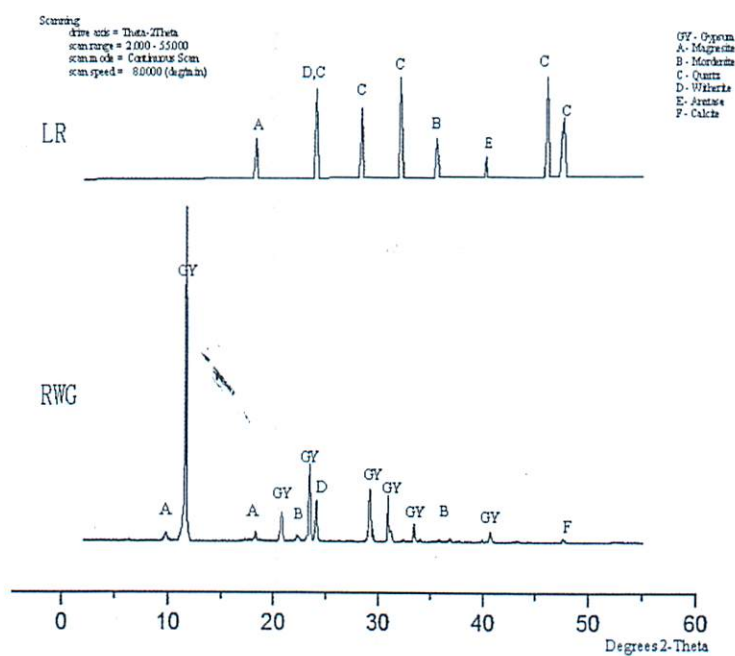
Fig. 13. XRD pattern of 10 g/L gypsum leached residue at 6.0 M HCl, 80°C, 400 rpm.
