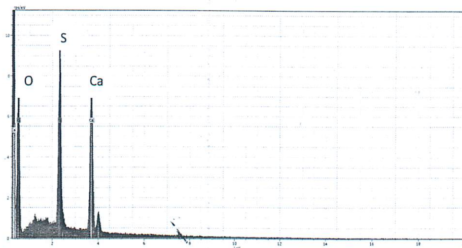
Fig. 3. Electron Dispersive Spectroscopy Spectrum of raw gypsum ore (RWG).
