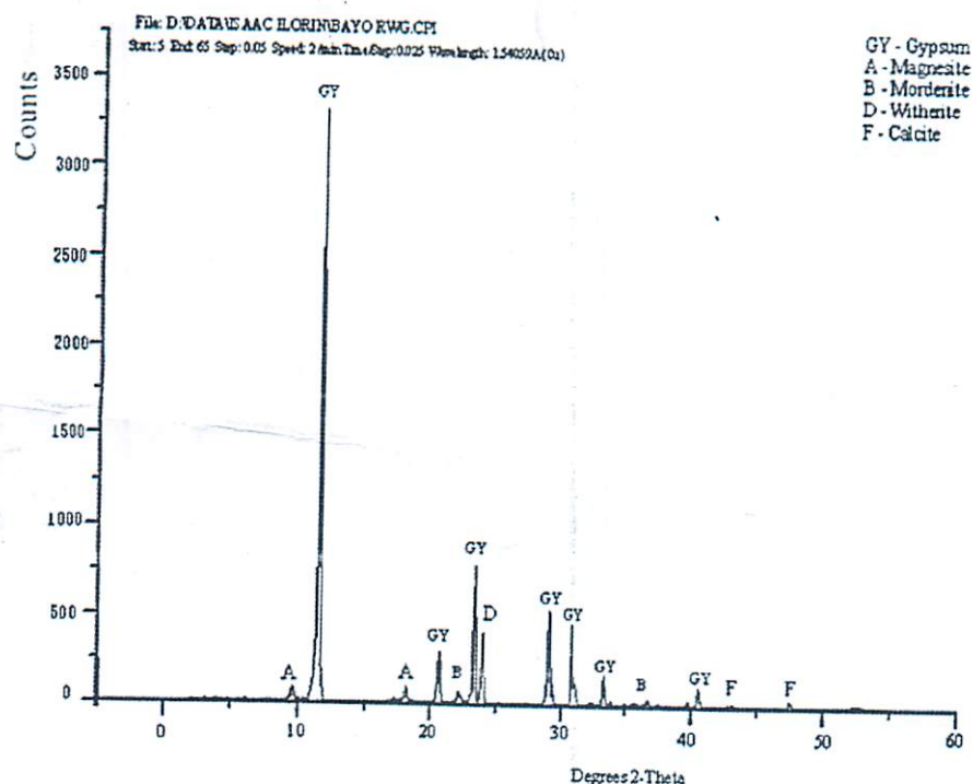
Fig. 1. XRD pattern of the gypsum ore sample showing different phases present with respective JCPDS file number used for peak attribution GY- Gypsum (01-070-0982), A-Magnesite (36-0383), B-Mordenite (49-0924), D- Witherite (5-0378), and F- Calcite (5-0586).
