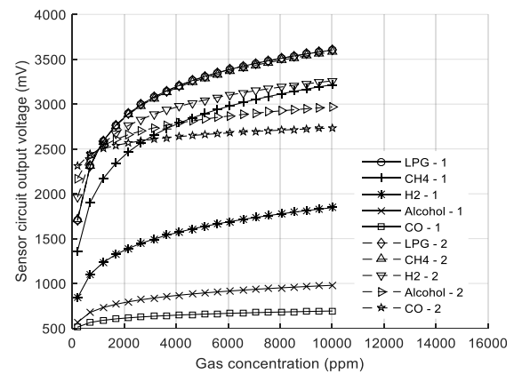
Figure 5. Plots of V_{RL} versus x for all MQ-6 gas sensor associated gases for R_L = 20 \text{ k}\Omega (solid line) and R_L = R_{L,MAX} (dash-dash line)
