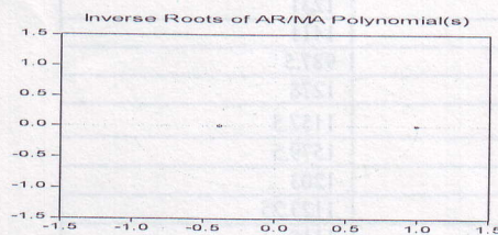
Fig. 2 Inverse Root of ARMA
