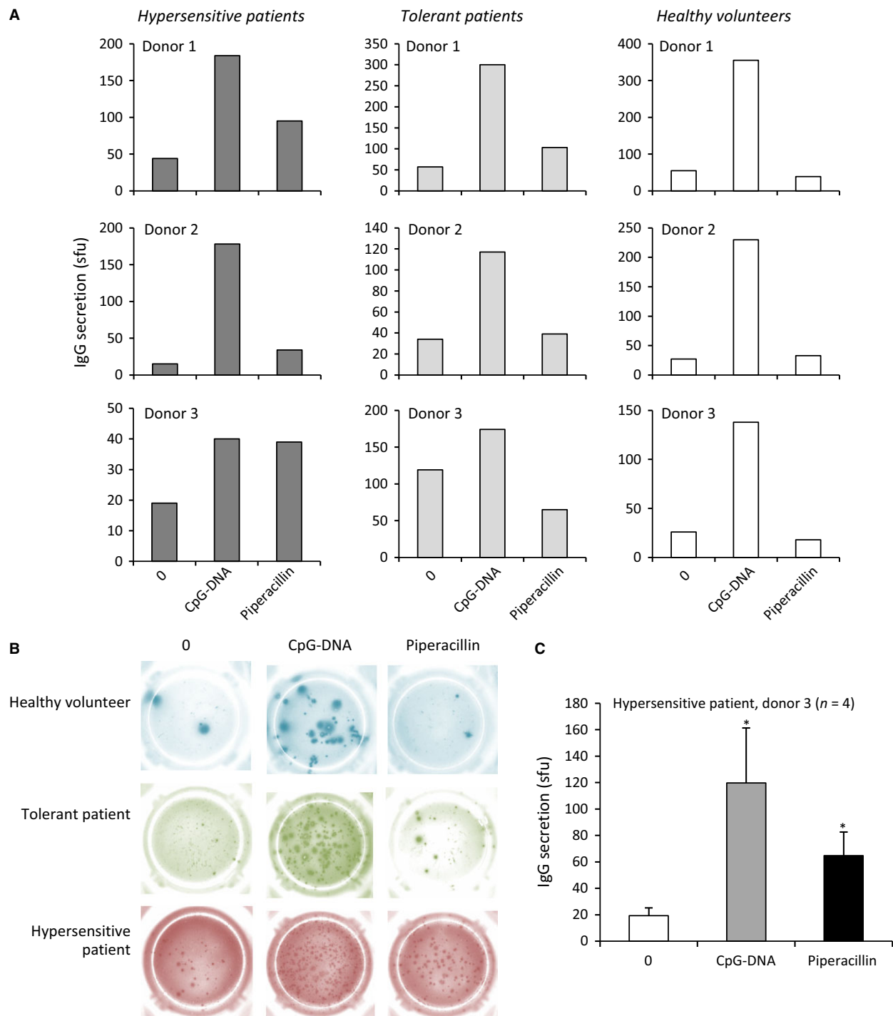
Figure 3 Piperacillin-specific IgG secretion from B cells of hypersensitive and tolerant patients and healthy volunteers. PBMC ( 1 \times 10^6/1 ml) were cultured in 24-well flat-bottomed plates with piperacillin (1–2 mM) and CpG-DNA (1.5 \mu g/ml) for 5 days. (A) ELISPOT plates were precoated with anti-human IgG incubated overnight at 4°C. PBMC were harvested and 5 \times 10^4 transferred to each well and incubated for 48 h. ELISPOT plates were developed according to the manufacturer's instructions. Data were analysed
