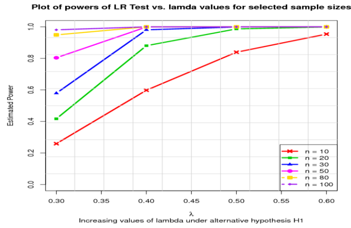
Fig 3.6: Plots of the powers of different LR tests at increasing values of parameter \lambda_1 under the alternative hypothesis H_1 for a fixed value of parameter \lambda_0 under the null hypothesis H_0 for different
