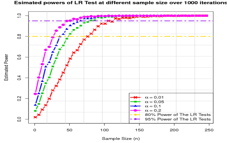
Fig 3.5: The plots of the estimated powers of the likelihood ratio tests at various sample sizes for some selected Type I error rates \alpha = 0.01, 0.05, 0.1, 0.2 for testing the hypothesis set H_0: f(x|\lambda = 0.2) vs. H_1: f(x|\lambda = 0.3) over 1000 iterations where x \sim \exp(\lambda) . The various graphs showed that the more the size \alpha of the LR test increases, the fewer the samples required by the test to achieve appreciable power.
