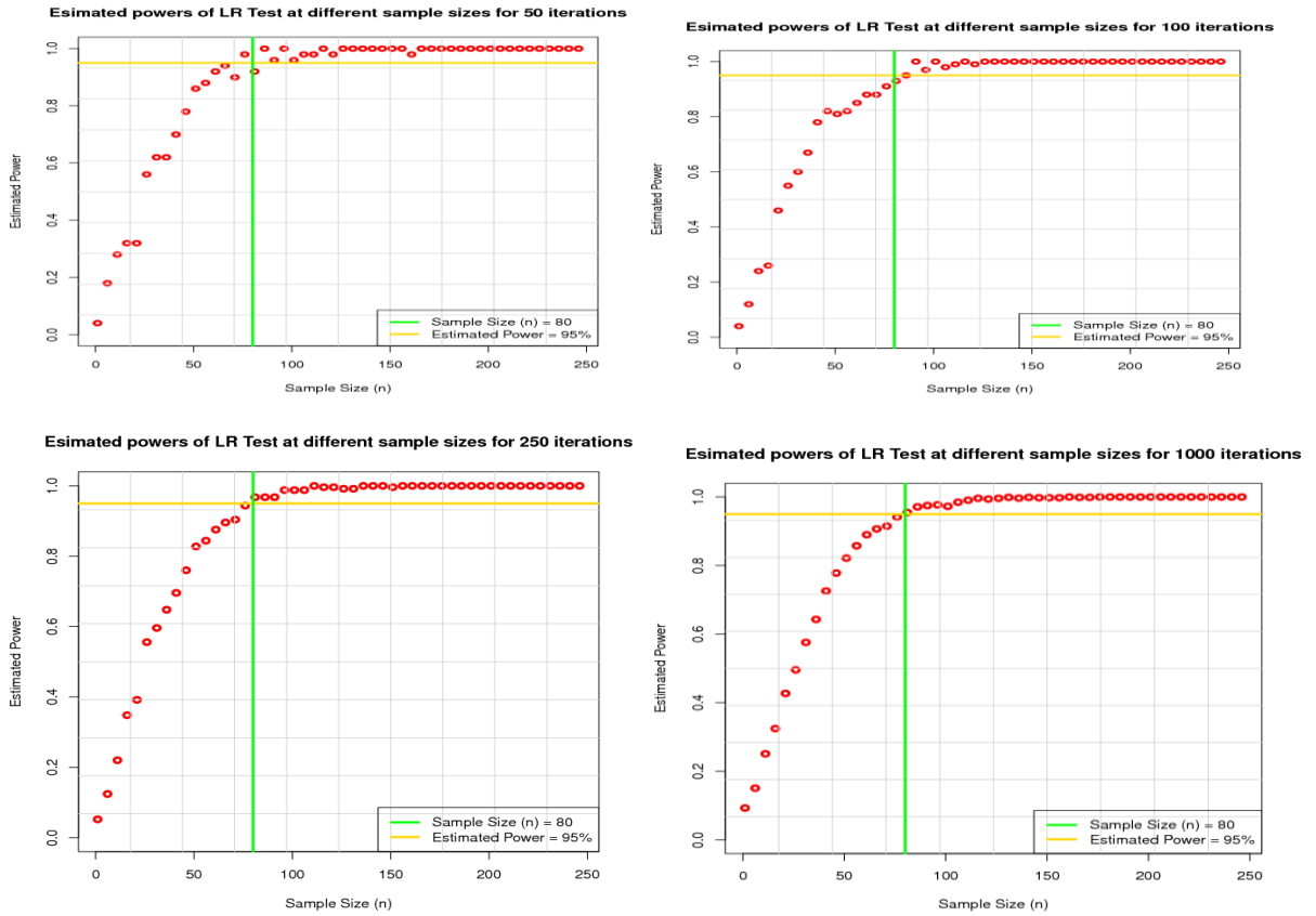
Fig 3.1: The graphs of the estimated powers of the likelihood ratio tests for the hypothesis set H_0: f(x|\lambda = 0.2) vs. H_1: f(x|\lambda = 0.3) , x \sim \exp(\lambda) , at various sample sizes and at 50, 100, 250 and 1000 iterations. The vertical green line in all the graphs indicates the sample size ( n = 80 ) at which the LR test achieves the same 95% power across the four levels of iterations.
