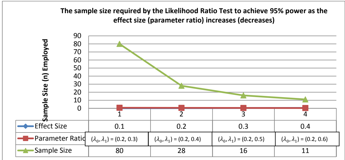
Fig 5.1: The graph showing the sample size requirements by the likelihood ratio test to achieve 95% power as the effect size of the test ( \Delta = |\lambda_0 - \lambda_1| ) increases for the hypothesis set H_0: \lambda = \lambda_0 vs. H_1: \lambda = \lambda_1 . In the four hypotheses considered, the value of parameter \lambda_0 of the exponential density under H_0 was set at 0.2 while that of \lambda_1 under H_1 were varied. Thus, the parameter pairs (\lambda_0, \lambda_1) = (0.2, 0.3) , (\lambda_0, \lambda_1) = (0.2, 0.4) , (\lambda_0, \lambda_1) = (0.2, 0.5) and (\lambda_0, \lambda_1) = (0.2, 0.6) with the respective effect sizes 0.1, 0.2, 0.3 and 0.4 were tested.
