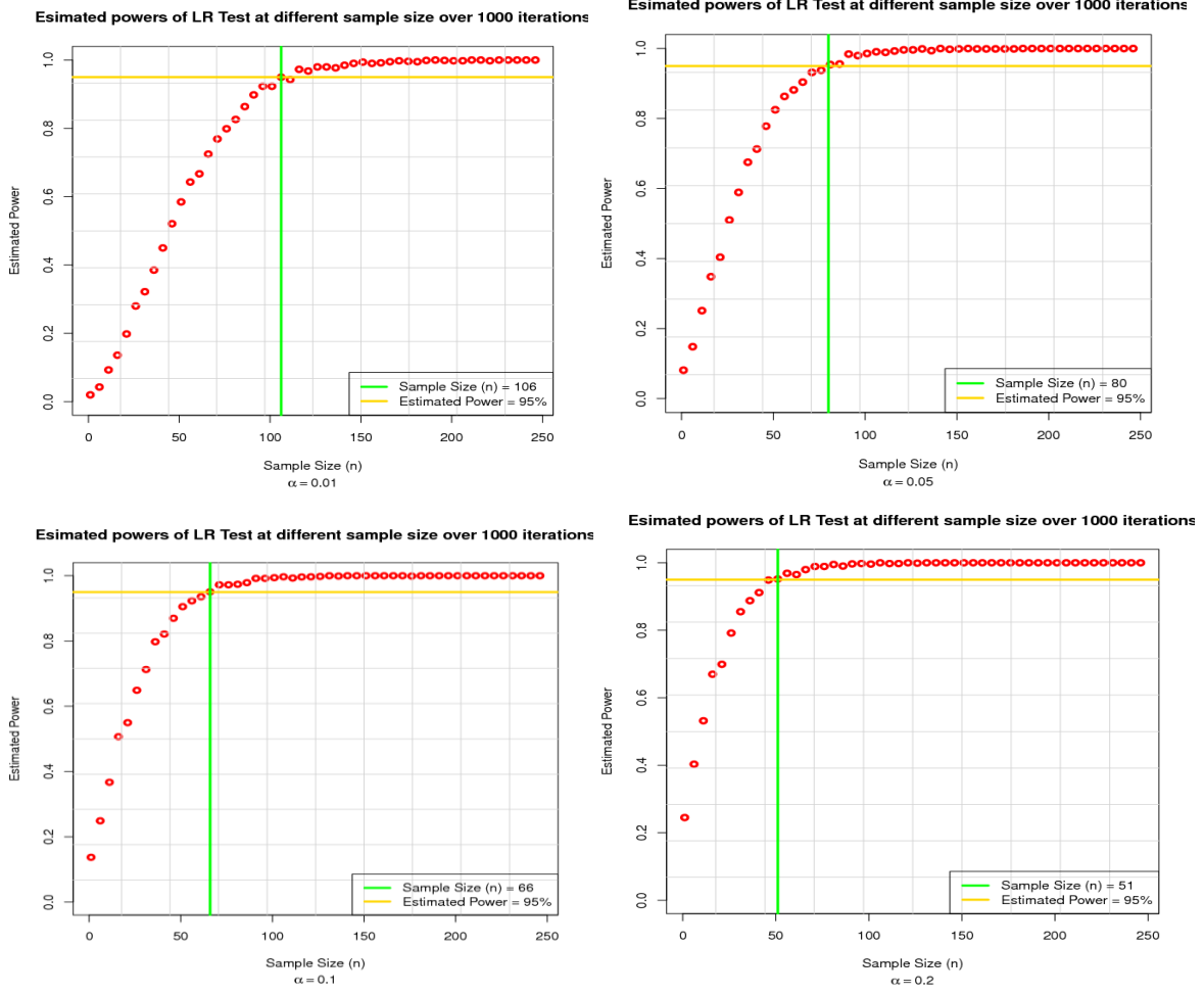
Fig 3.4: The plots of the estimated powers of the likelihood ratio tests at various sample sizes and at some selected Type I error rates \alpha within the interval (0,1) for testing the hypothesis set H_0: f(x|\lambda = 0.2) vs. H_1: f(x|\lambda = 0.3) over 1000 iterations where x \sim \exp(\lambda) . The vertical green line in each graph indicates the sample size at which the LR test achieves 95% power. The four graphs showed that fewer samples are required by the LR test to achieve 95% power as the chosen significance level \alpha increases (from 0.01 to 0.2).
