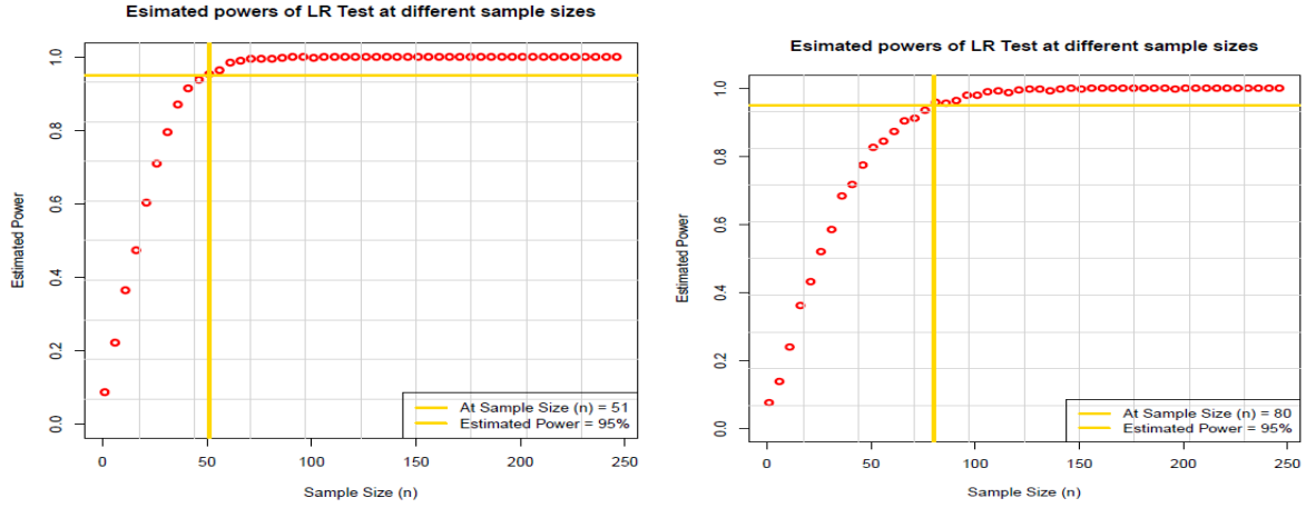
Fig H_0: \lambda = 0.3 vs. H_1: \lambda = 0.5 , \Delta = 0.2 , R = 3/5 H_0: \lambda = 0.4 vs. H_1: \lambda = 0.6 , \Delta = 0.2 , R = 2/3 hypotheses set with equal effect size \Delta = |\lambda_0 - \lambda_1| = 0.2 but at varying parameter ratios R = \frac{\lambda_0}{\lambda_1} over 1000 iterations (LR tests). The vertical golden line in each graph indicates the sample size at which the LR test achieves about 95% power. The sample size required (indicated by vertical golden line in each graph) by the LR test to achieve 95% power increases as the value of the parameter ratio R decreases even with equal effect size of 0.2 across the various tests.
