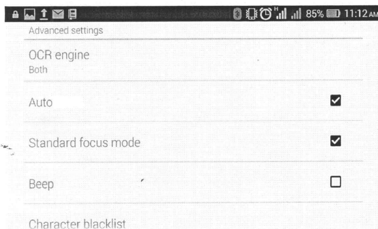
Figure 8: Settings Page
