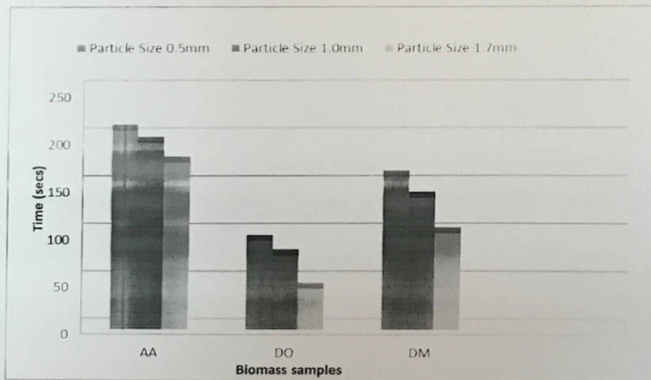
Figure 5: Water resistance test on the pellet samples of different particle sizes produced with binder
