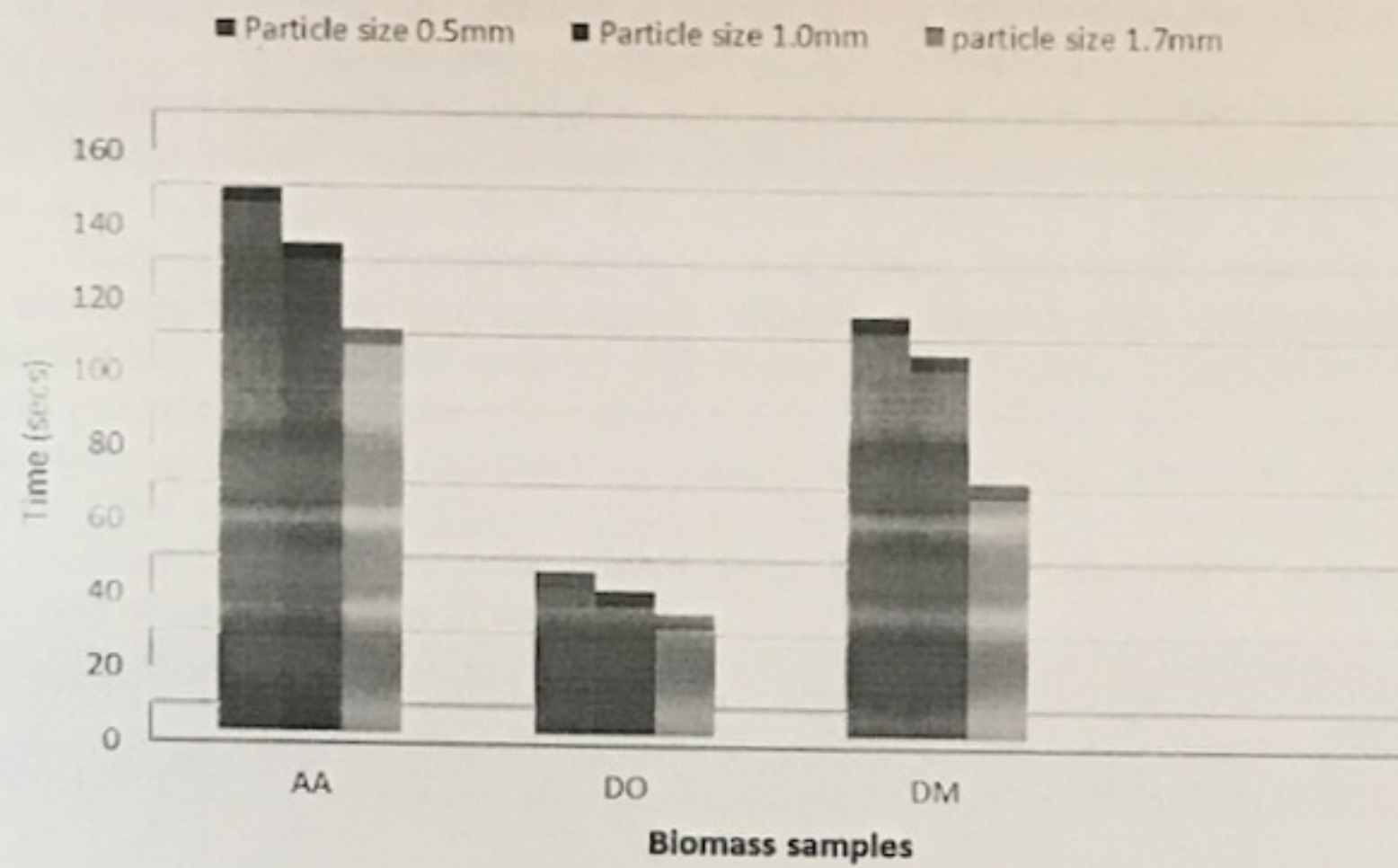
Figure 4: Water resistance test on pellet samples of different particle sizes produced without binder
