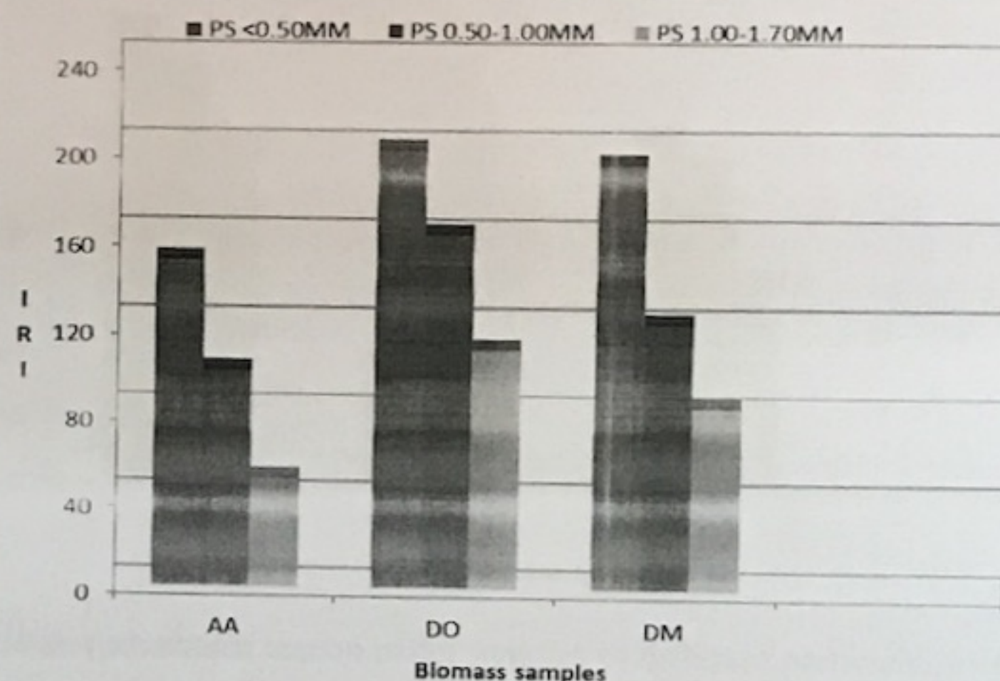
Figure 2: Impact resistance index (IRI) for pellet samples produced without a binder
