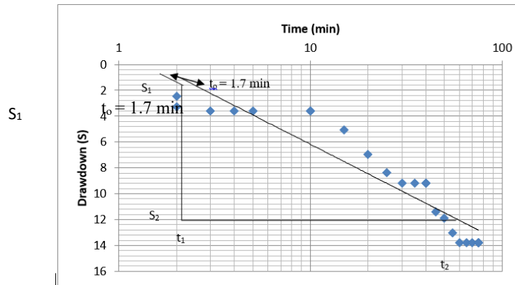
Figure 7: Plot of drawdown versus time for Reke waterside
