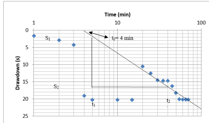
Figure 9: Plot of drawdown versus time for Amayo waterside
