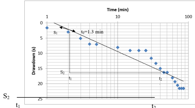
Figure 8: Plot of drawdown versus time for Ganmo waterside
