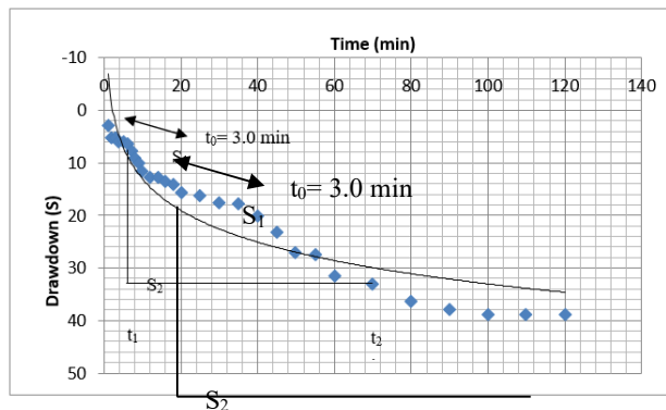
Figure 12: Plot of drawdown versus time for Budo-Ojoku waterside
