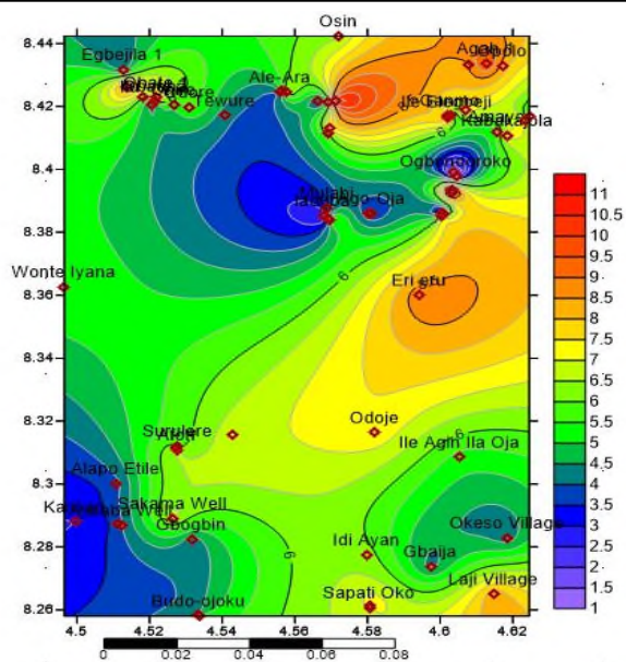
Figure 5: Groundwater level map at the end of the rainy season
