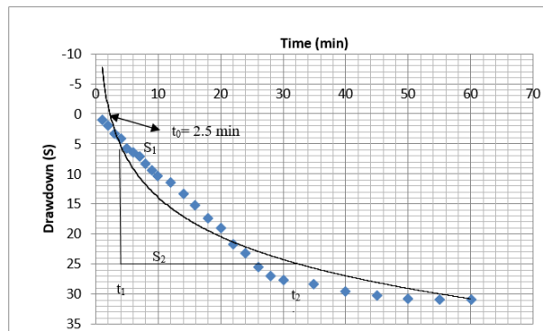
Figure 10: Plot of drawdown versus time for Osin- Aremu waterside
