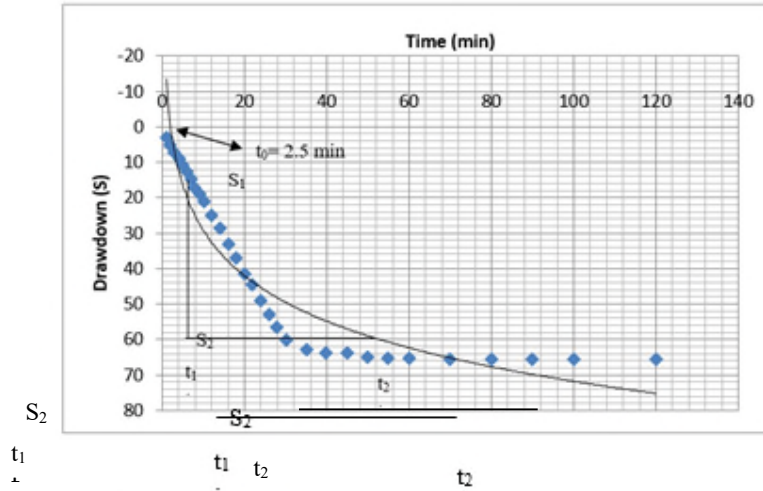
Figure 11: Plot of drawdown versus time for Ita - Elepa waterside
