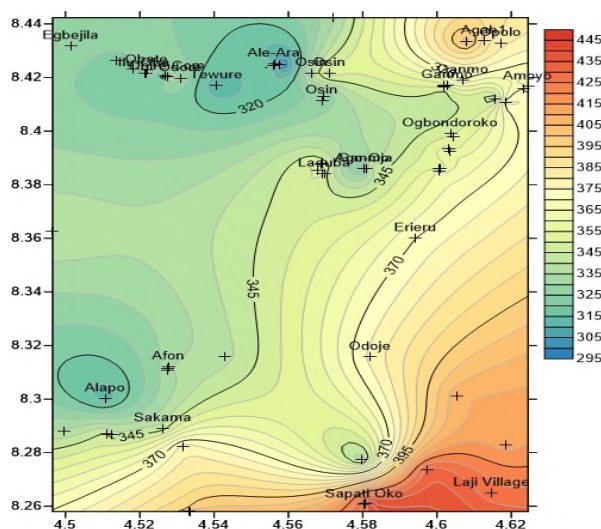
Figure 2: Groundwater contour map at the end of the rainy season
