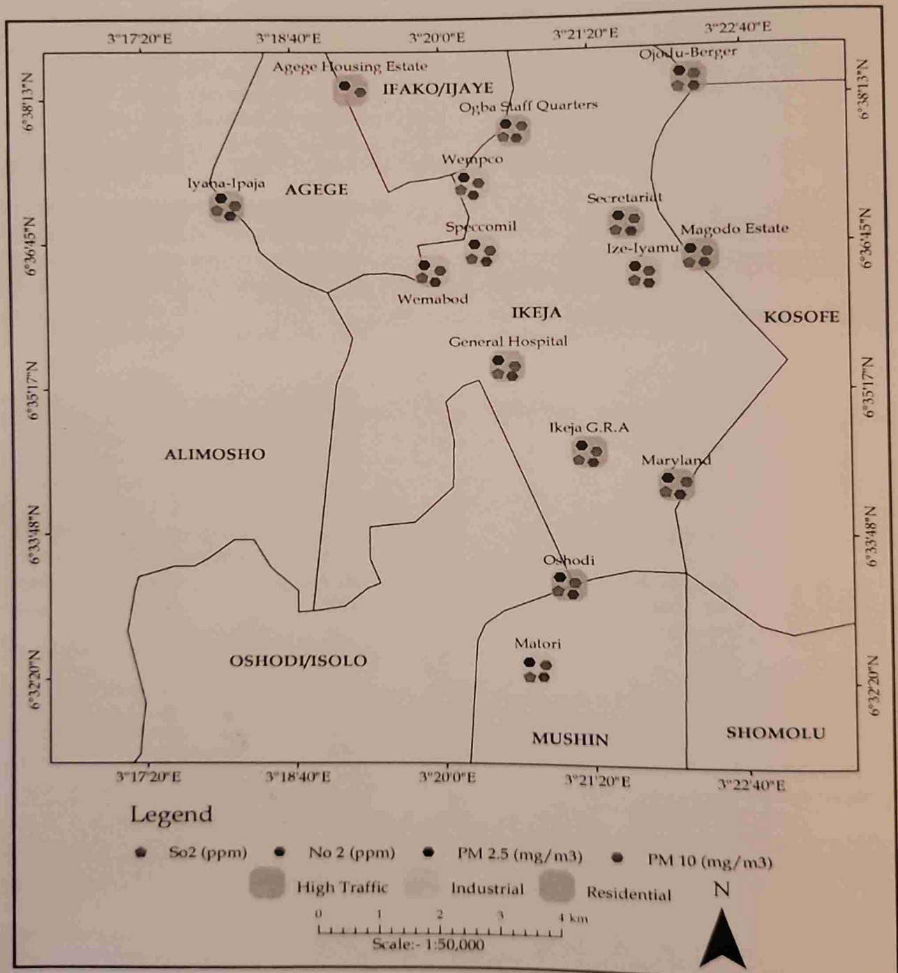
Figure 3: Spatial pattern of Hotspot areas of pollutants
