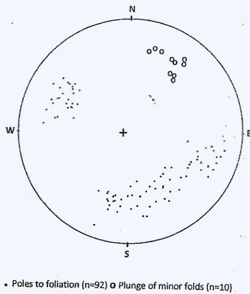
Fig. 4: Stereonet plots around the synformal structure
