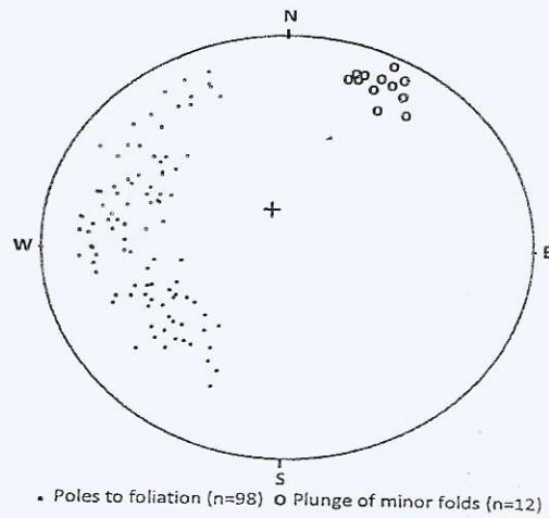
Fig. 3: Stereonet plot around the overturned fold
