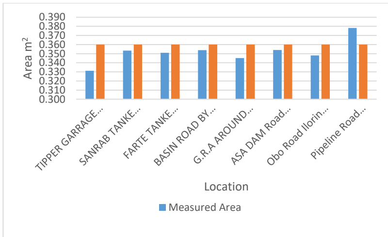
Figure 1: Graphical representation of measured area and standard area
