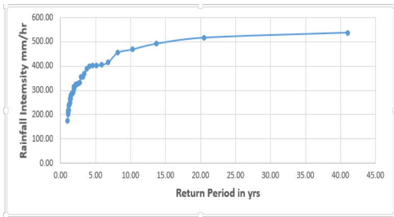
Figure 2: Frequency analysis for 2 years return period.
