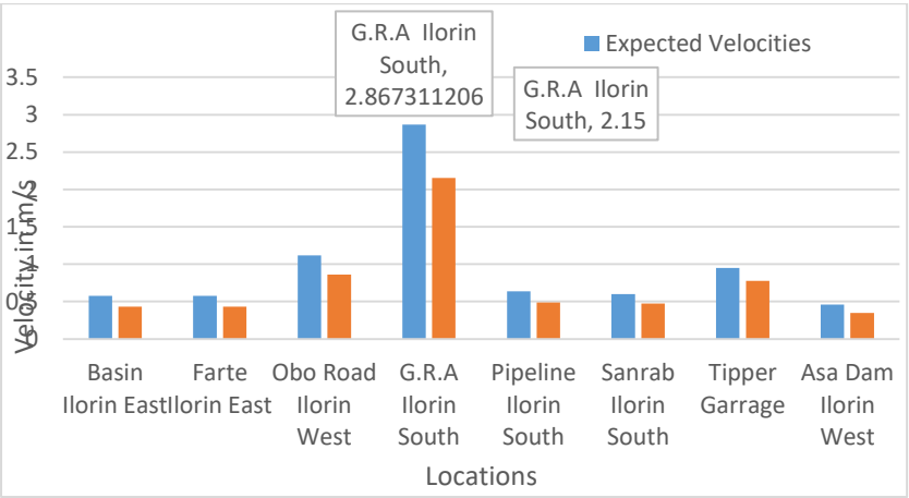
Figure 6: Graphical Representation of the observed and expected velocities
