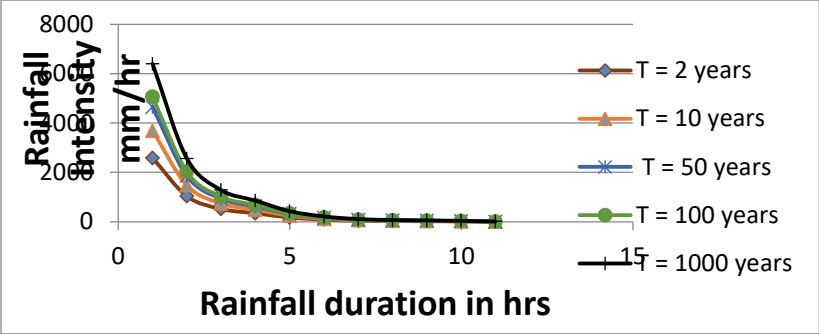
Figure 3: IDF curve for various return periods
