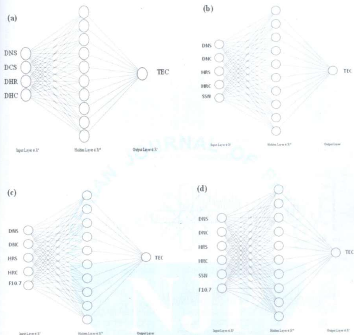
Figure 2: Schematic diagram of proposed neural network models. (a) NN1 model, (b) NN2 model, (c) NN3 model, (d) NN4 model.
