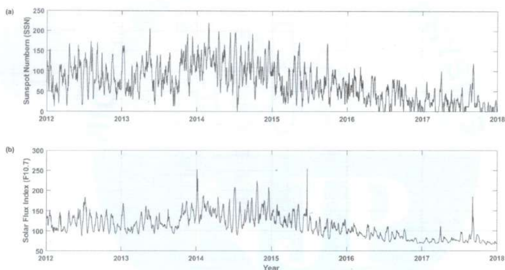
Figure 4: The solar activity indices between 2012 to 2017 (a) daily averages of SSN (b) daily average of F10.7.
