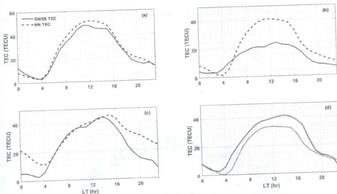
Figure 6: Comparison of observation GNSS TEC value with NN TEC value for some selected days (a) 17 th March 2014 (b) 6 th June 2016 (c) 18 th September 2015 and (d) 6 th December 2015
