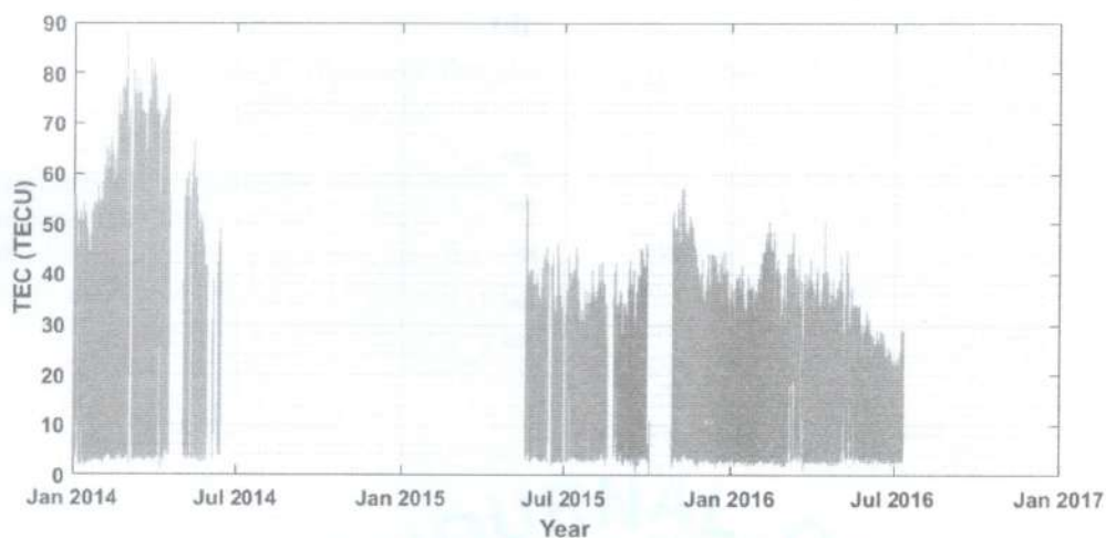
Figure 3: The variation of TEC between 2014 to 2016
