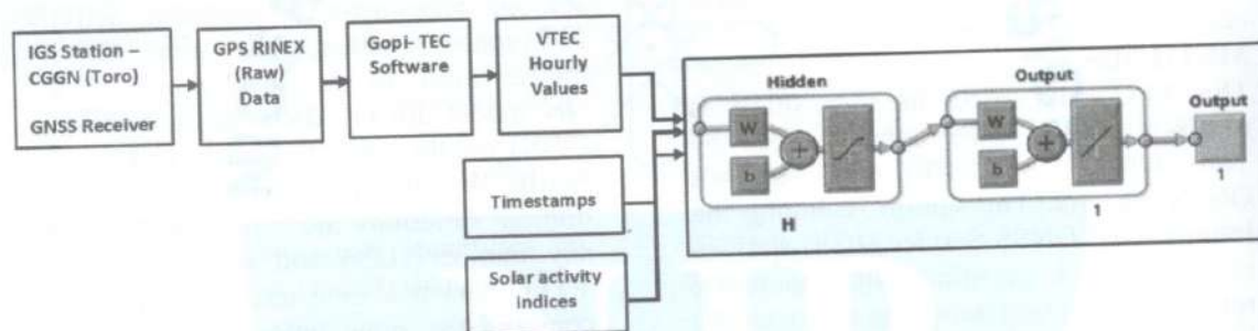
Figure 1: The flow process of the NN model on MATLAB
