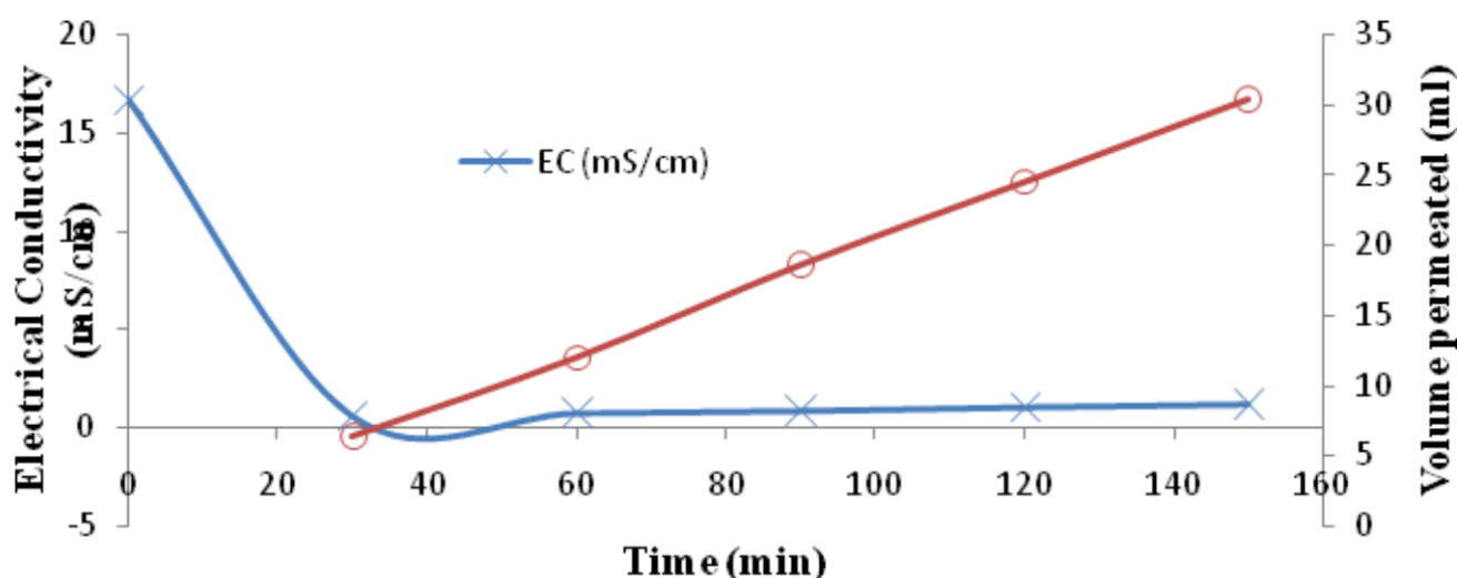
Fig. 6. Variation of conductivity with desalination time in hyper-saline water
