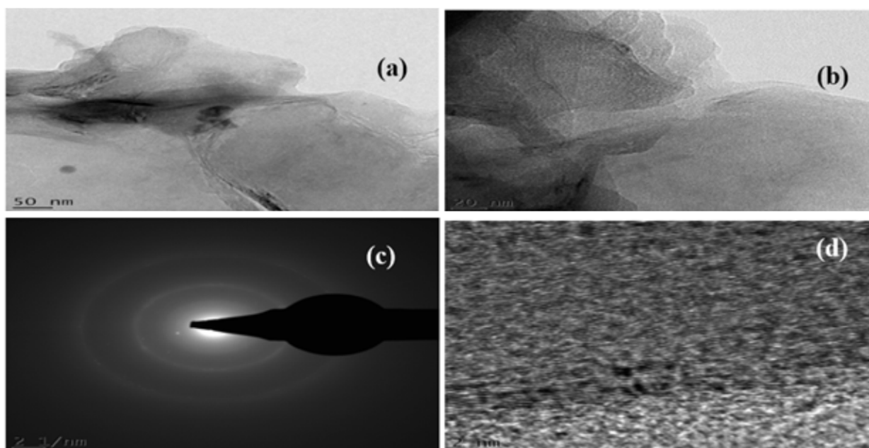
Figure 1. TEM images of graphene/graphene oxide produced from electrochemical exfoliation of ZCBs showing (a),(b) evidence of few-layer graphene nanomaterial, (c)the SAED pattern,and (d) lattice fringes/arrangement of carbon atoms in the graphene sheet.
