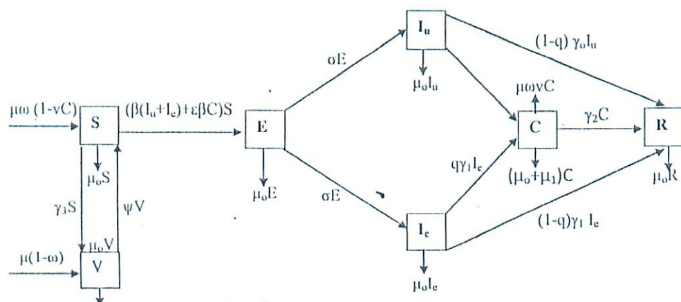
Fig. 2.1: Flow diagram of HBV transmission
