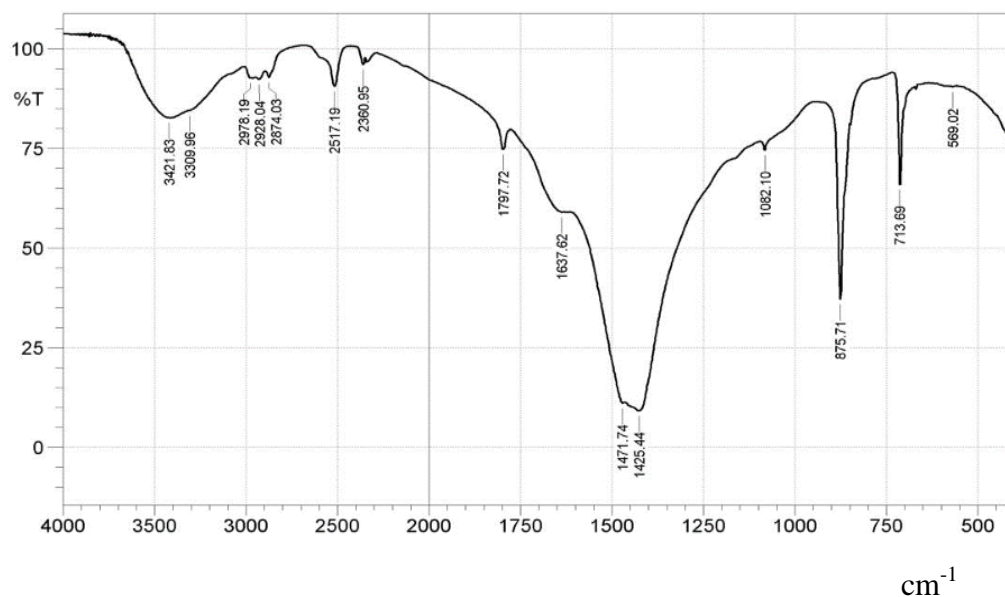
Figure 3: FTIR Spectra of Chicken Eggshell
