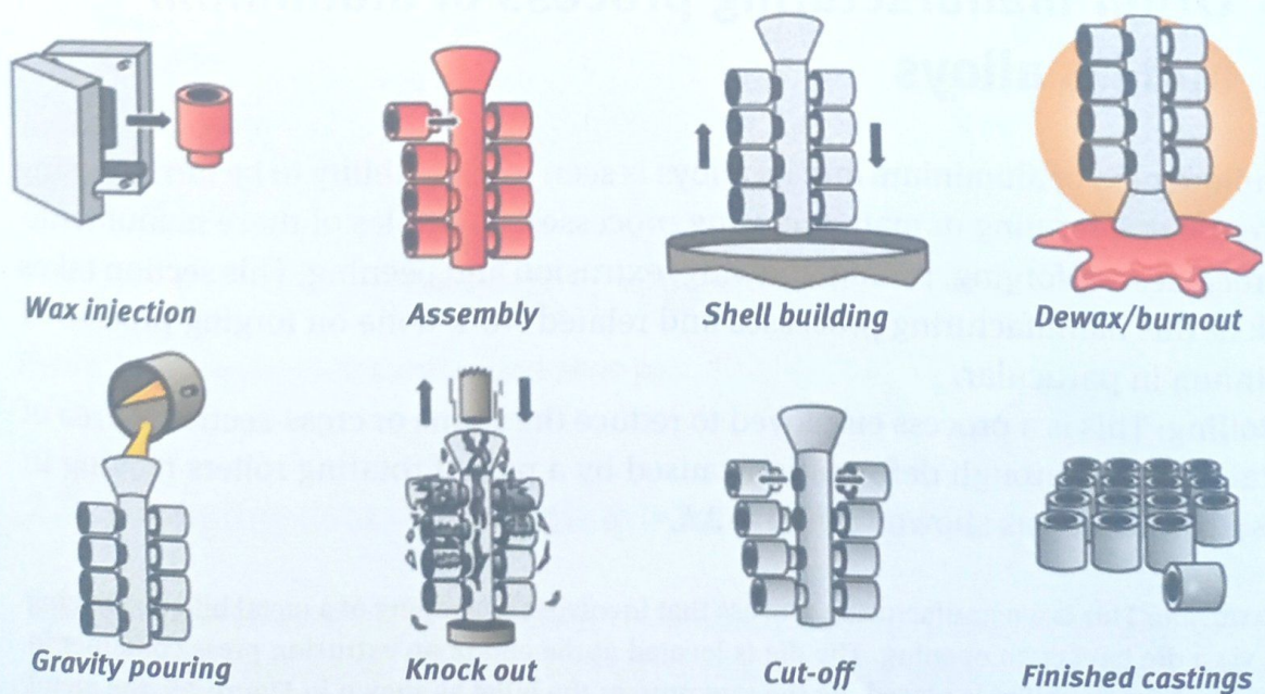
Figure 2.3: Basic steps in investment casting process [9].
