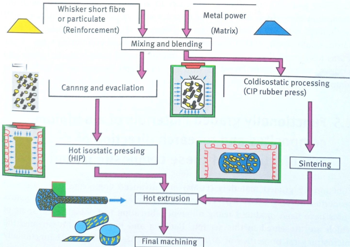
Figure 2.9: Steps for powder metallurgy processing route [26].
