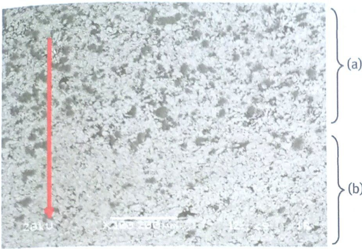
Figure 2.12: Transition zone from (a) 10 wt% \text{Al}_2\text{O}_3 reinforced material to (b) Al2124 alloy [43].
