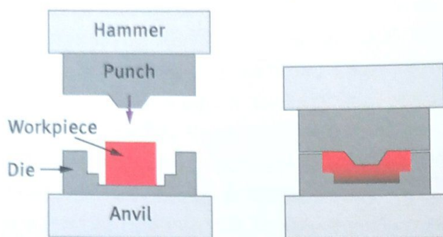
Figure 2.6: Hammer forging of a metal piece [15].
