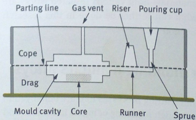
Figure 2.2: Mould for sand casting [8].
