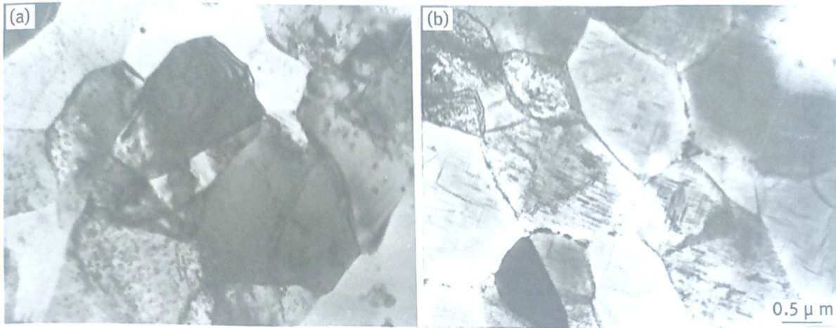
Figure 2.1: Aluminium alloy microstructure in (a) as-quenched state and (b) aged at 473 K for 20 h.
