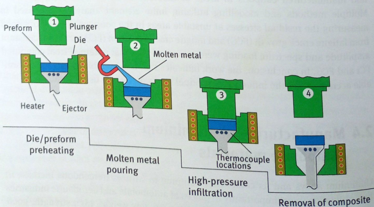
Figure 2.7: Squeeze casting of discontinuously reinforced composites [26].
