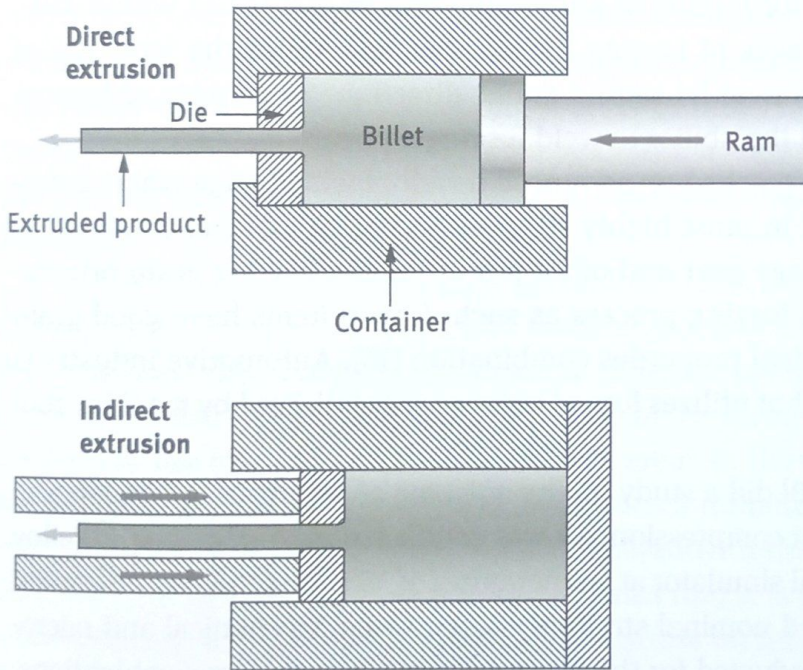
Figure 2.5: Extrusion process of a metal billet [14].
