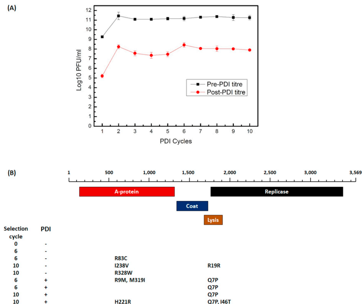
Fig. 5. Selection of PDI-resistant MS2. (A) Figure shows infectivity titre of MS2 before and after TMPyP-PDI treatment. Each PDI cycle was subjected to 0.5 \mu M TMPyP and illuminated at 32 mW.cm -2 for 30 s. As a control, a sample of MS2 was passaged serially in the absence of TMPyP for 10 cycles ( n = 3 \pm S.D.). (B) Viral genomic RNA was extracted from recovered passages 0, 6 and 10. RNA was reverse-transcribed into cDNA and cloned into transient vector pCR-Blunt. Colony clones of individual genomes of wild-type, TMPyP-PDI treated and non-treated cycle passages 6 and 10 were purified and sequenced. Sequence reads were aligned against reference MS2 sequence (NC_001417.2). Figure shows a cartoon annotation of the MS2 (NC_001417.2) genome. The cartoon shows open reading frames (ORFs) of the A-protein (red), coat protein (blue), lysis protein (green) and replicase (black). Mutations identified are listed below respective open reading frames. The mutation at nucleotide 1697 resulted to a synonymous coat protein mutation (S121S), and a non-synonymous lysis protein mutation (Q7P). (For interpretation of the references to colour in this figure legend, the reader is referred to the web version of this article.)
