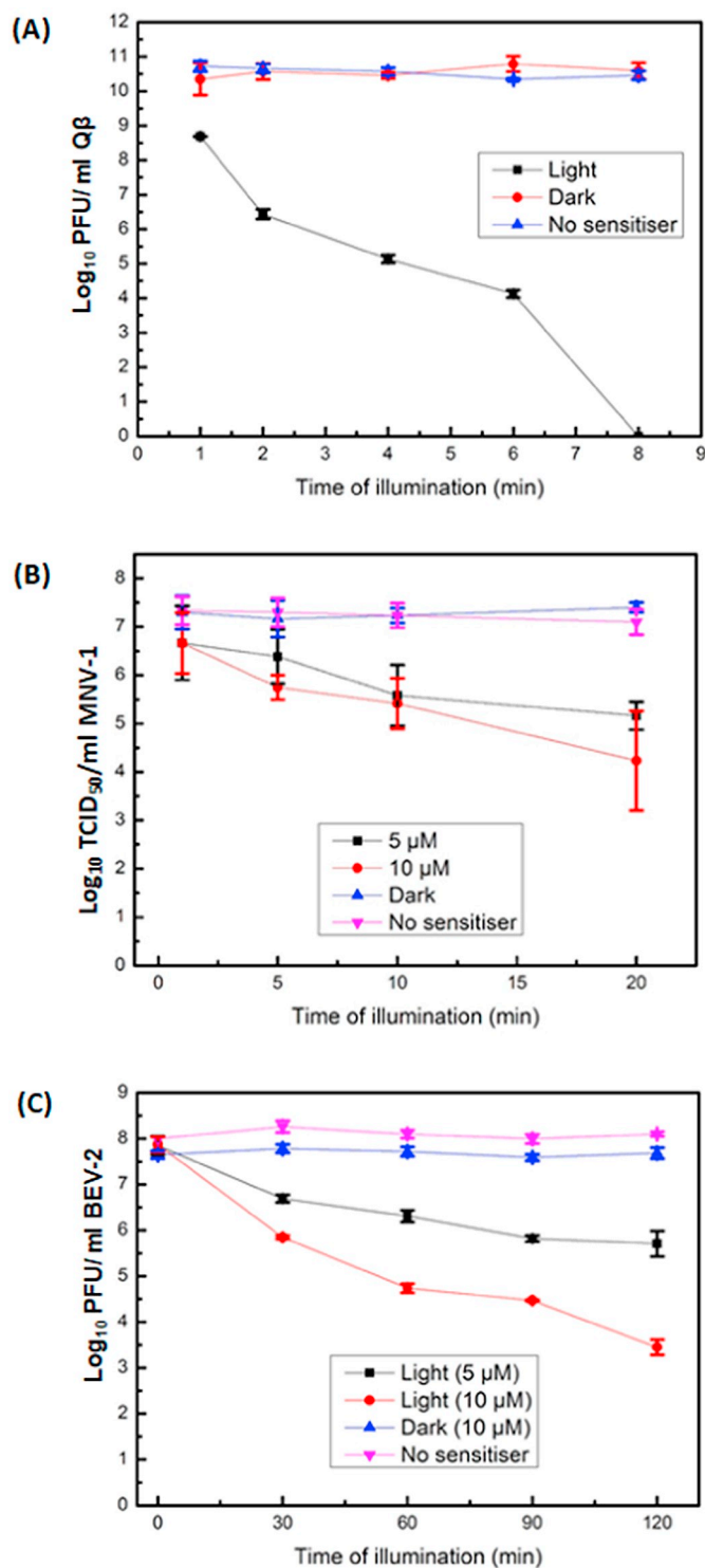
Fig. 2. PDI of icosahedral viruses over time. The samples were and illuminated at 32 mW cm -2 . The figure shows PDI kinetics of (A), Q \beta Virus samples treated with 0.5 \mu M TMPyP; (B), MNV-1 treated with 5 \mu M and 10 \mu M TMPyP; (C), BEV-2 treated with 5 \mu M and 10 \mu M TMPyP. The dark controls were treated with the concentration of photosensitizer shown but not illuminated whilst no photosensitiser controls (NS) were illuminated without photosensitizer present. n = 3 \pm S.D.
