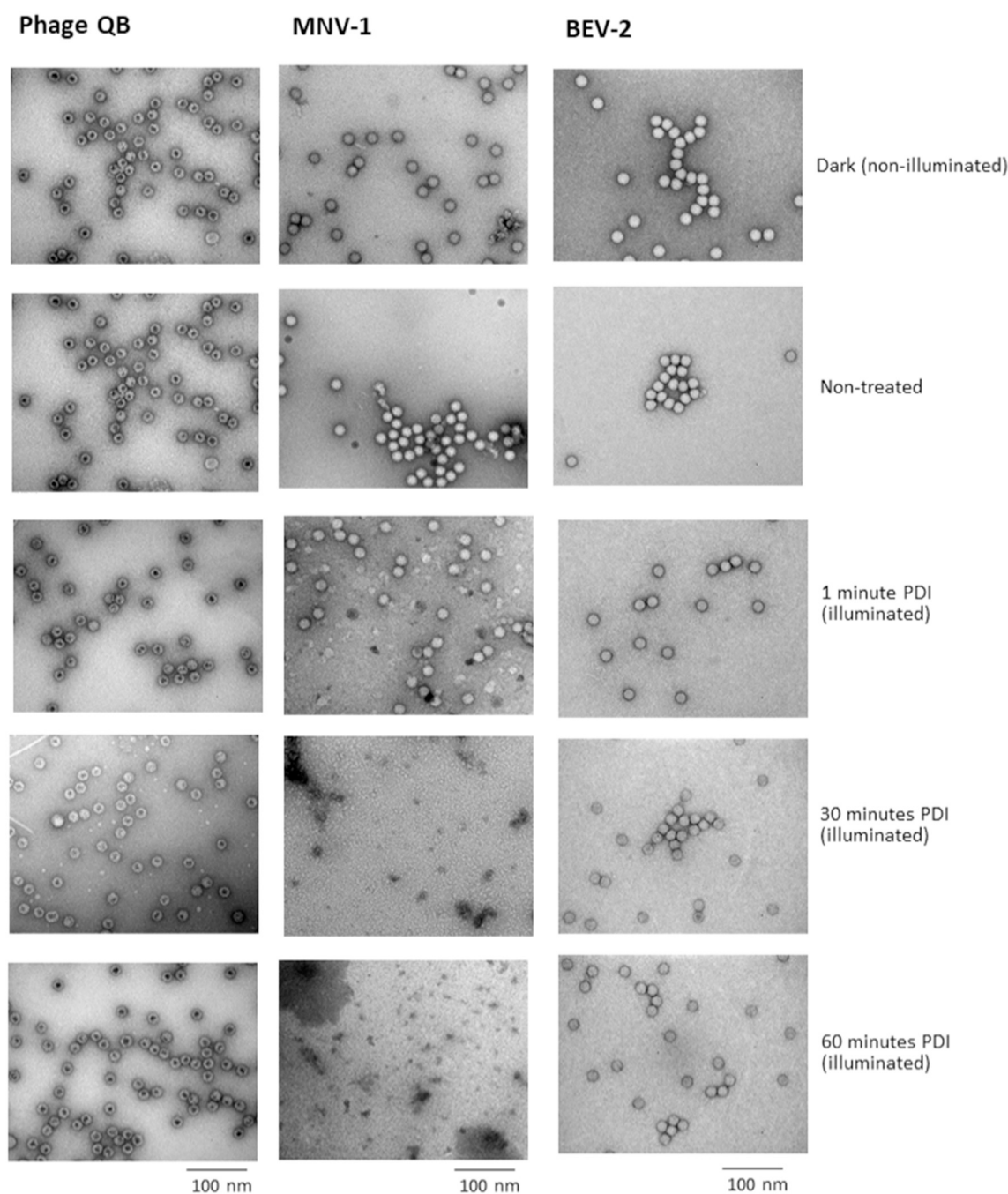
Fig. 3. TEM of PDI treated model viruses with 50 \mu\text{M} TMPyP in solution. Samples of QB, MNV-1 and BEV-2 were purified through sucrose gradients and dialysed into TEM buffer as described in Methods. Dialysed virus samples were treated with 50 \mu\text{M} TMPyP and illuminated at 32\text{ mW cm}^{-2} for a range of durations from 1 min to 60 min. As controls, “Dark experiments” were also treated with 50 \mu\text{M} TMPyP but incubated for 60 min. Treated samples were immediately stained with 1% (w/v) uranyl acetate and visualised by TEM. Figure shows negatively stained TEM micrographs of QB, BEV-2 and MNV-1, respectively. Sample treatments are indicated on the right-hand panel. Scale bars are shown underneath each micrograph column.
