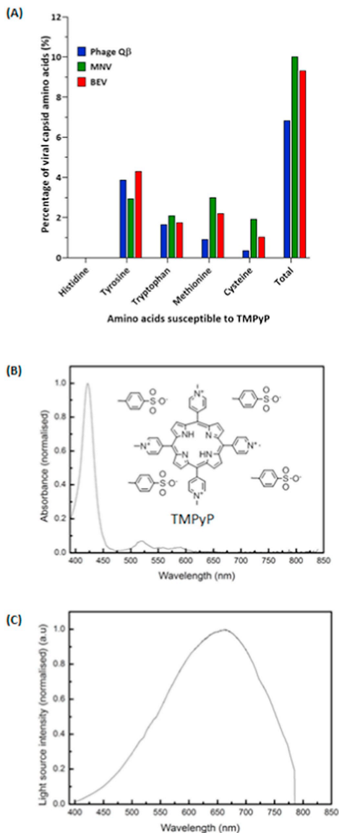
Fig. 1. Spectral properties of PDI light source and absorption spectra of TMPyP, and amino acids most susceptible to singlet oxygen mediated oxidation among model viruses. (A) Percentage of the capsid protein residues that are most susceptible to PDI among the icosahedral viruses studied. Reference sequences of bacteriophages MS2 (NC_001417.2), and Qβ (AY099114.1), MNV-1 (KR349276.1) and BEV-2 (AY508697.1) were accessed from the NCBI genebank and assessed for abundance of tryptophan, histidine, methionine, cysteine and tyrosine within the capsid region. Figure also shows the percentage abundance of a combination of all five amino acids susceptible to singlet oxygen mediated oxidation. (B), light spectra of our PDI light source (Schott KL 2500 LCD, Schott Ltd., UK). The PDI light source spectra (400 nm–786 nm) showed that this mainly emitted visible light including some near infrared. The spectral peak is between 641 nm - 661 nm; (C), absorption spectra of the photosensitiser-TMPyP used for PDI of the viruses. The absorption peak of TMPyP is 422 nm. The TMPyP chemical structure was from ChemACX.com, ChemDraw Pro 13.0.
