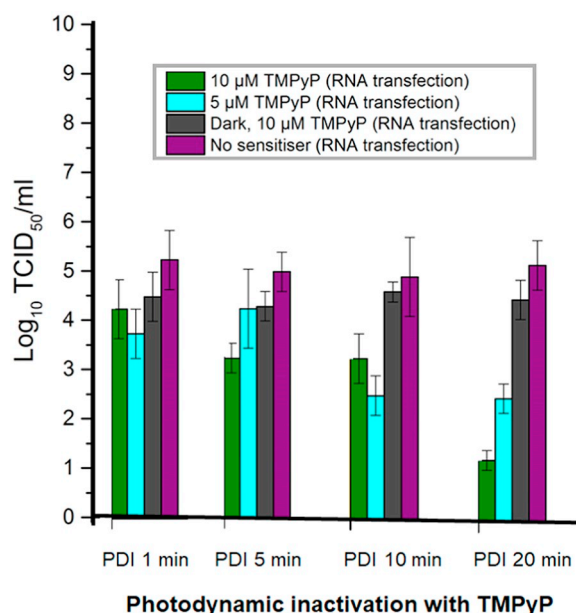
Fig. 4. The effect of TMPyP-PDI treatment on RNA infectivity of MNV-1. Samples of MNV-1 were treated with 5 \mu M and 10 \mu M TMPyP and illuminated at 32 mW cm -2 for up to 20 min. Viral RNA was extracted from these samples and transfected into RAW 264.7 cells. Recovered viral infectivity titres were determined by TCID 50 assays. As controls, “dark” samples were treated 10 \mu M TMPyP in the absence of light illumination, while “no sensitizer” samples (NS) were illuminated in the absence of TMPyP ( n = 3 \pm S.D.).
