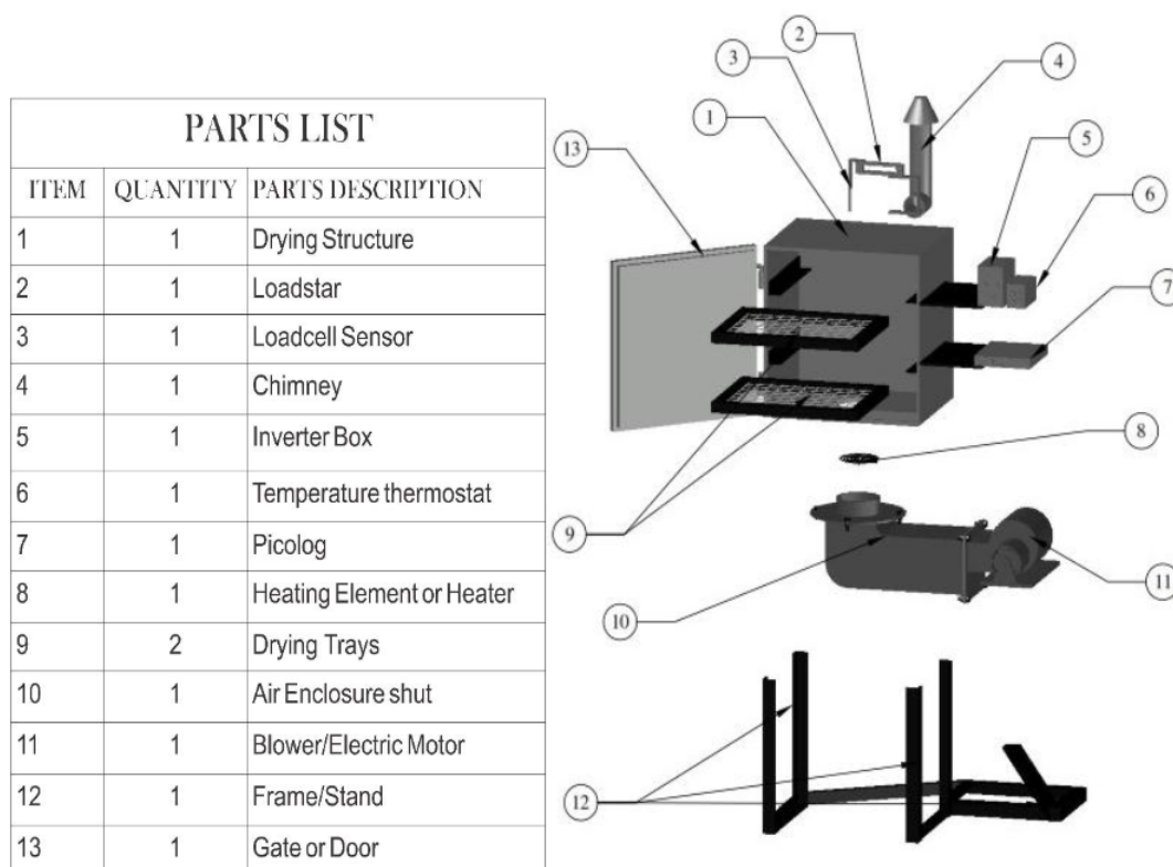
Figure 1 Exploded diagram of dryer with associated instrumentation
