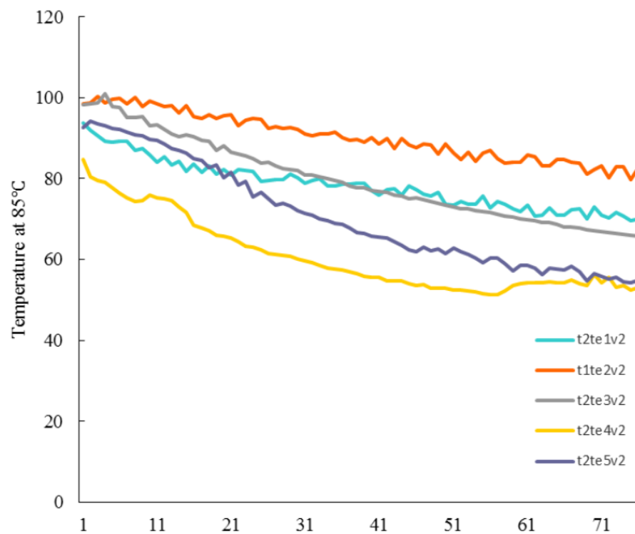
Figure 10 At velocity 2.5 m s -1
