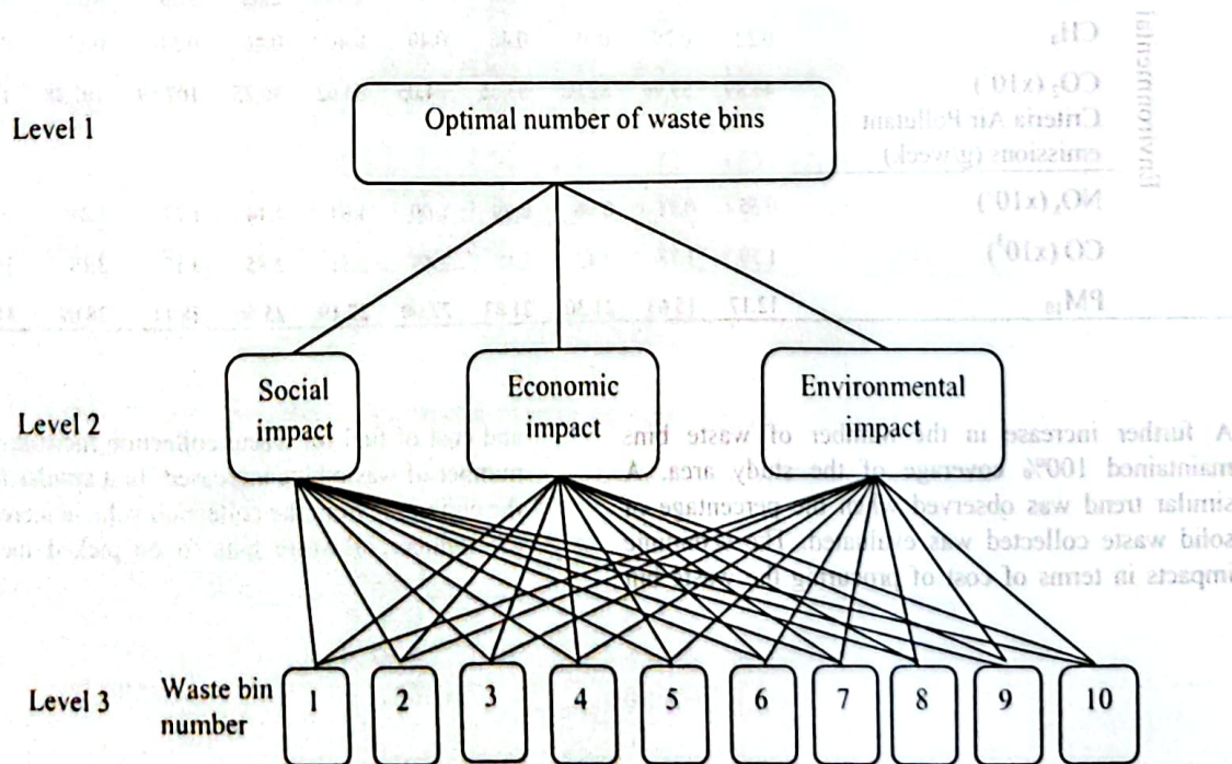
Figure 2 Different levels of hierarchy in the AHP model
