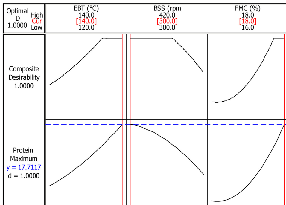
Fig. 5. Numerical optimization of extrusion parameters for protein-rich brown rice-water melon seeds extruded snacks.
