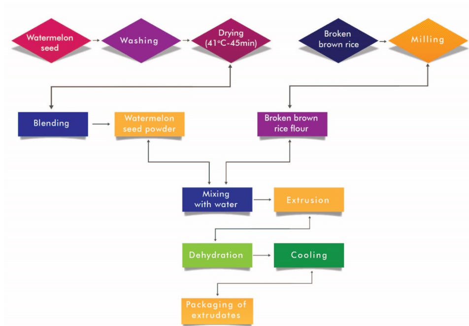
Fig. 1. Flow chart for the production of brown rice-watermelon seeds extruded snacks.
