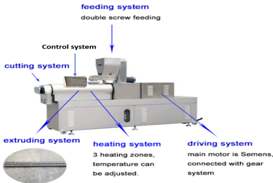
Fig. 2. Schematic of a typical co-rotating twin-screw extruder.
