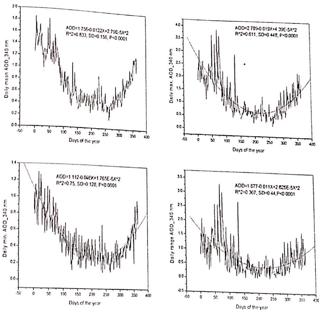
Figure 3: Fit for the variation of yearly representation of Daily mean, maximum, minimum, and range for AOD at 340 nm for Ilorin for year 2002-2014.
