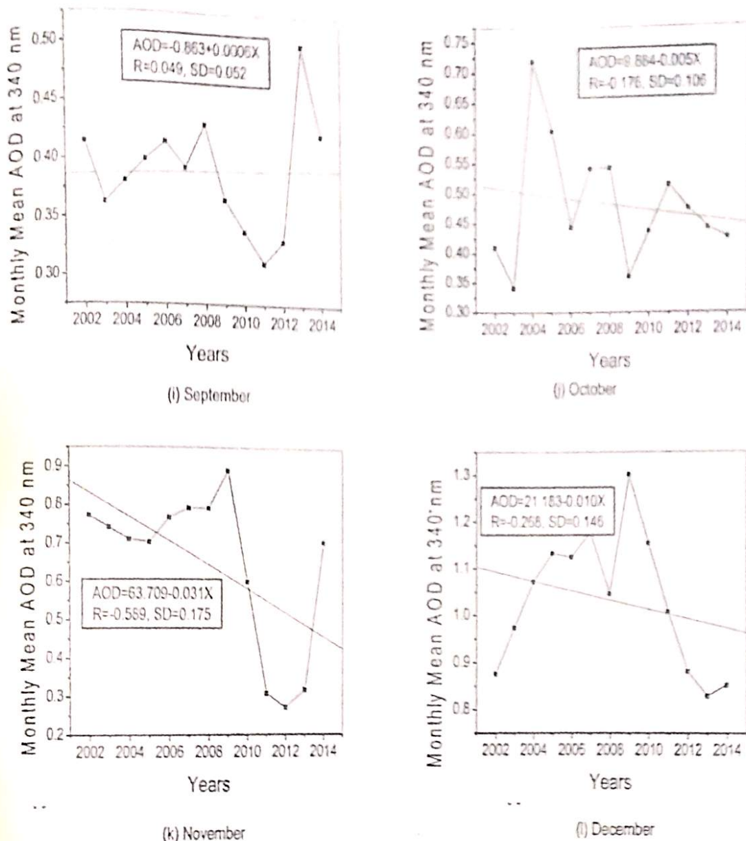
Figure 7 (a)-(l): Linear regression trends of monthly mean of yearly AOD 340 nm at Ilorin from January to December for 2002-2014.
