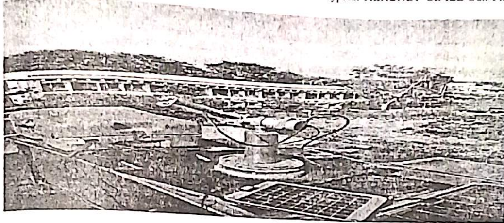
Figure 2: AERONET CIMEL Sun-photometer at block 9 of the faculty of physical science, University of Ilorin, Nigeria.
