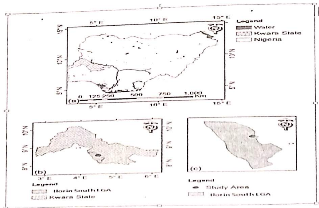
Figure 1: Digitized (a) Map of Nigeria showing Kwara State (b) Map of Kwara State showing Ilorin South LGA (c) Map of Ilorin South LGA showing study area
