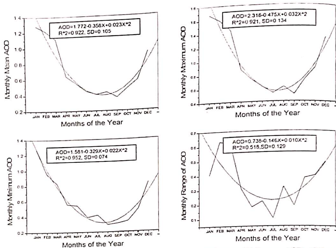
Figure 4: Fit for the variation of monthly mean, maximum, minimum and range of daily mean AOD at 340 nm for Ilorin for year 2002-2014.
