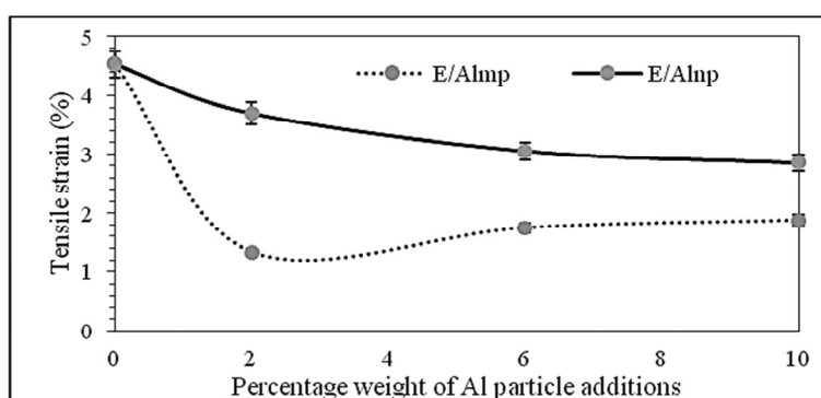
Figure 7. Tensile strain of the epoxy/aluminium composites
