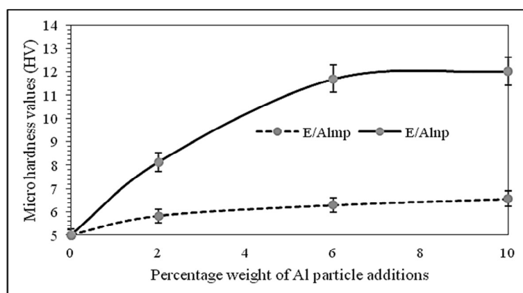
Figure 9. Micro hardness of the epoxy/aluminium composites
