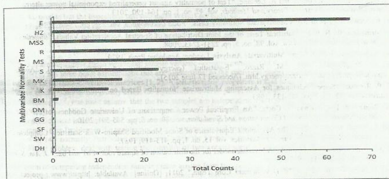
Figure 4: Bar Chart Showing Summary of Number of Times Type 1 Error Rates Approximate True Level of Significance
