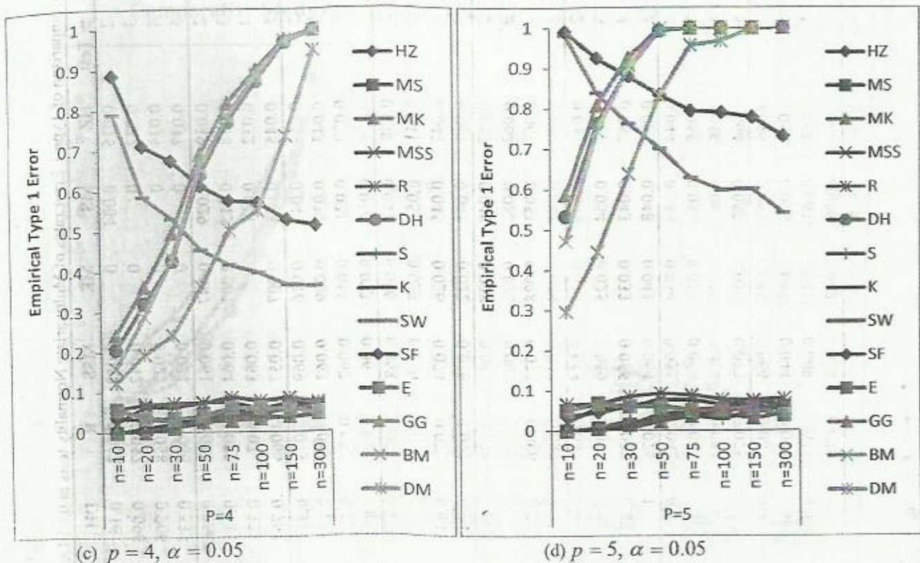
Figure 2: Comparison of Type 1 Error rate of Different Normality Tests at \alpha = 0.05
