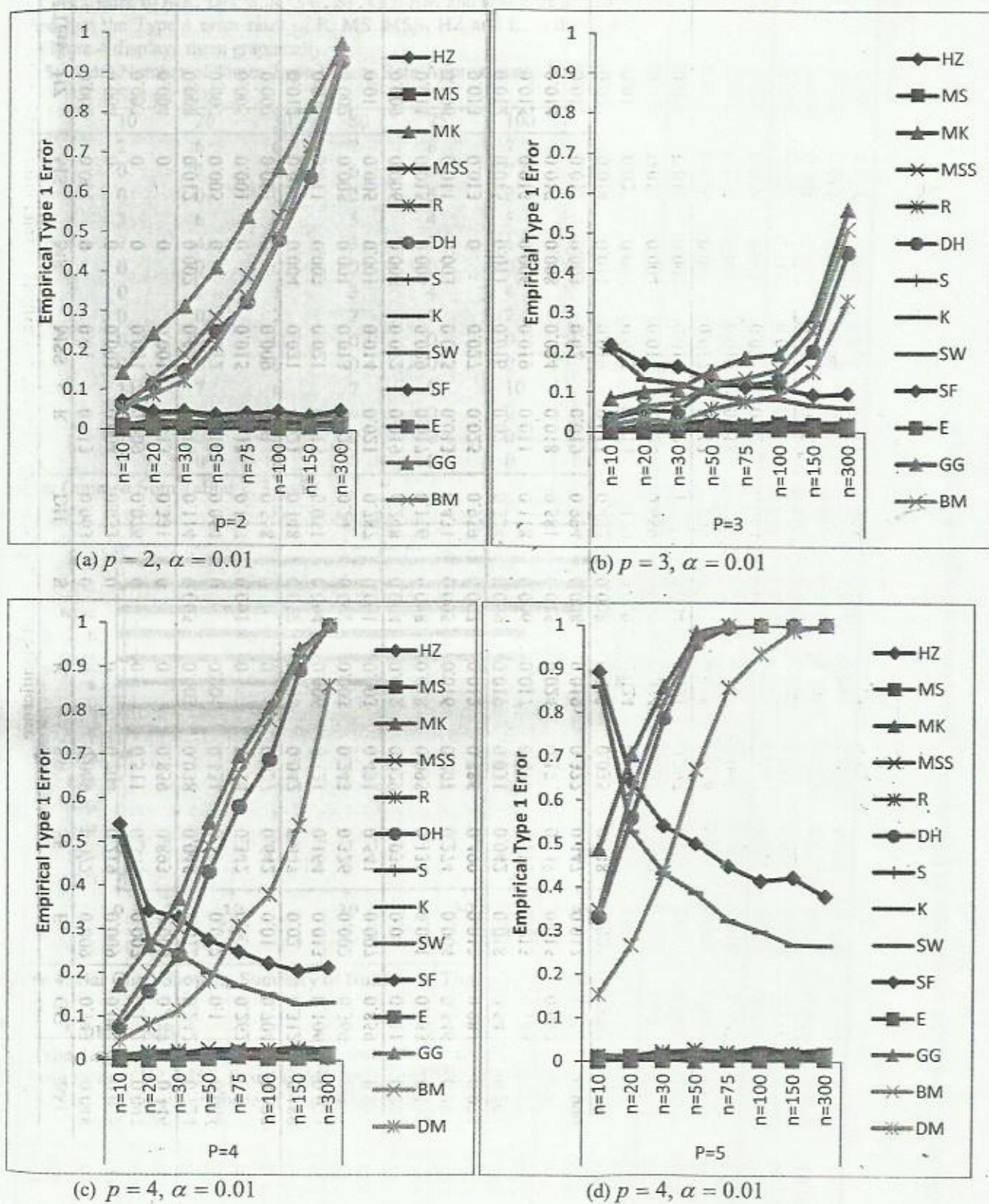
Figure 3: Comparison of Type 1 Error rate of Different Normality Tests at \alpha = 0.01
