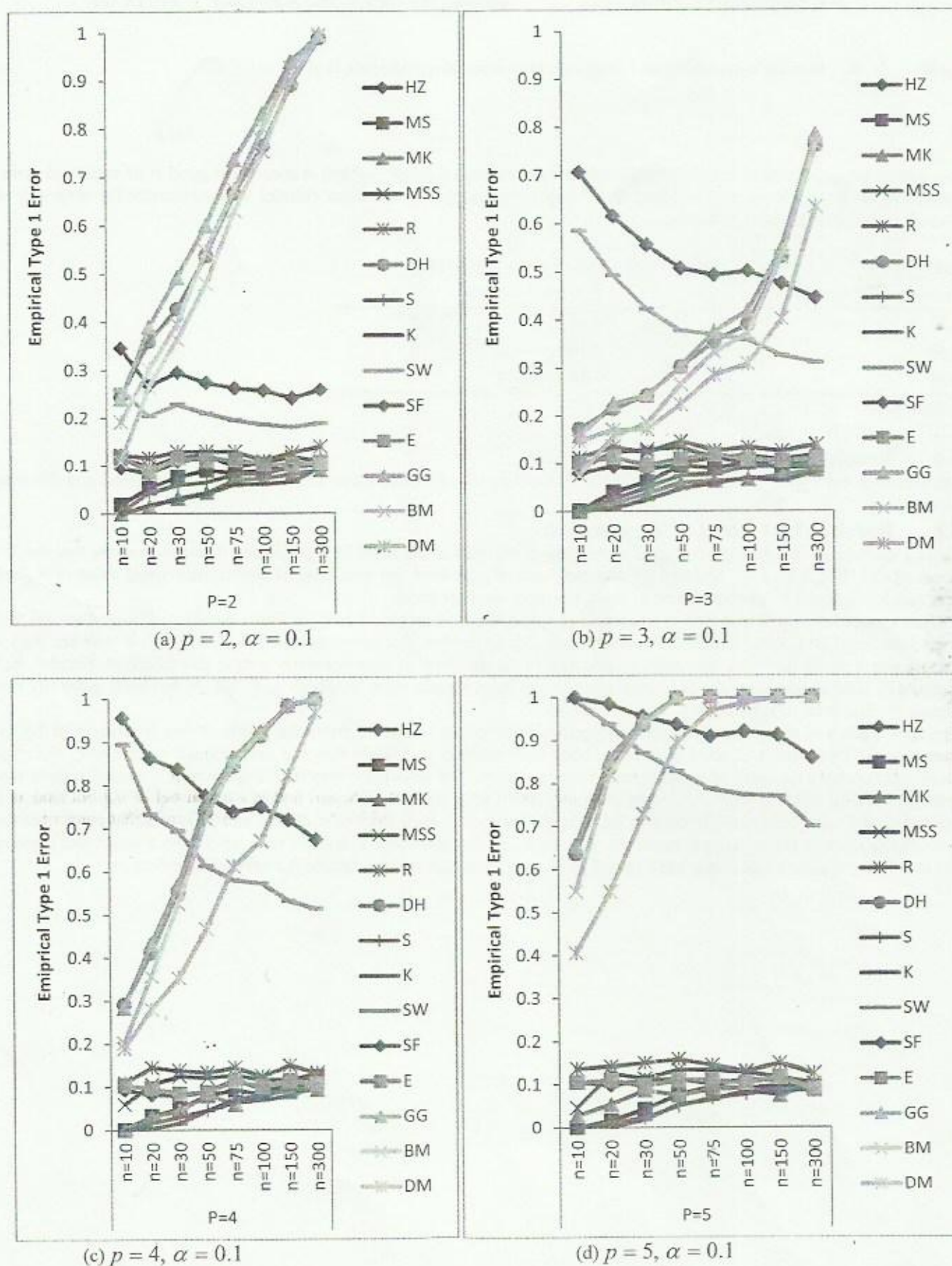
Figure 1: Comparison of Type 1 Error rate of Different Normality Tests at \alpha = 0.1
