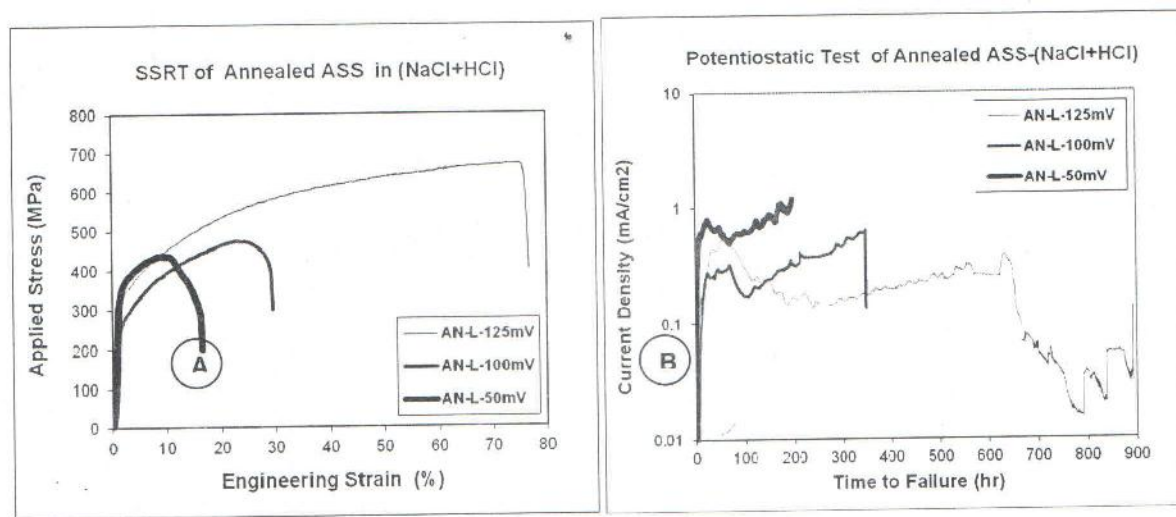
Figure 2: SSRT Curves for Samples Tested at Strain Rate of 2.4 \times 10^{-7} \text{s}^{-1} , pH of 1.5, and Applied Potentials of -125mV, -100mV and -50mV at 25°C: Applied Stress Vs Strain (A) and Current Density Vs Time to Failure (B)
